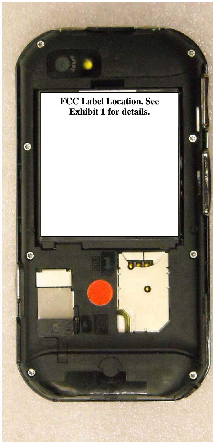
Figure 3-7. Interior Compartment of radio
