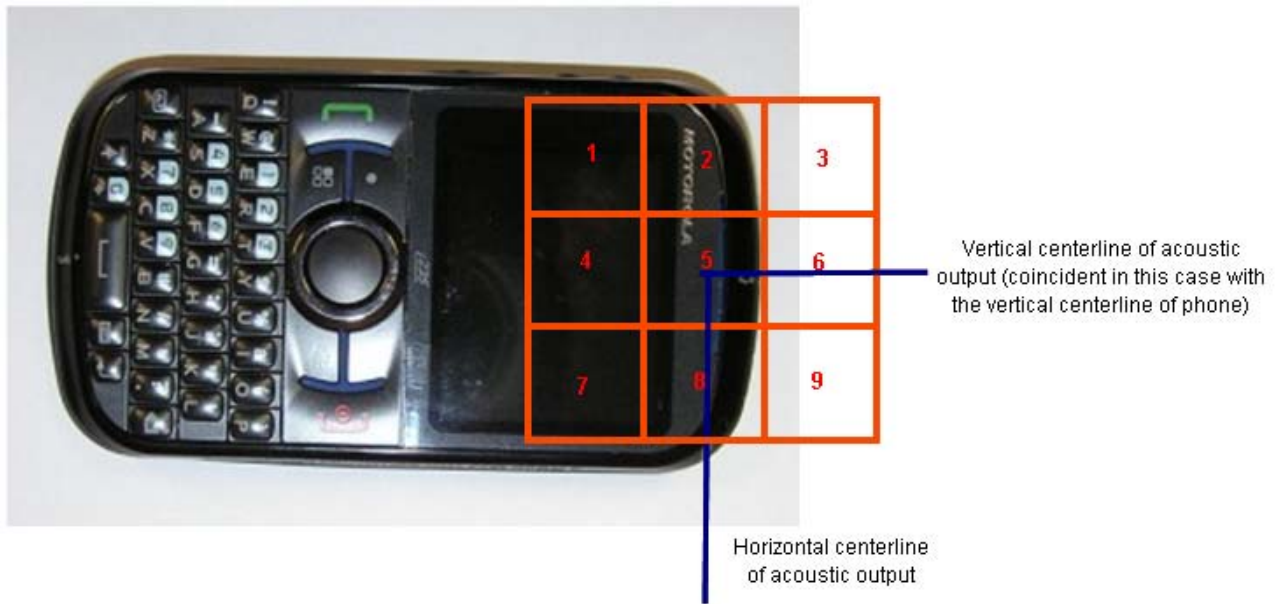
Figure 2. Phone Open - Orientation and Measurement Plane for RF Emissions Testing
