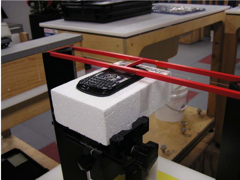
Figure 3. Positioning and Measurement for RF Emissions
