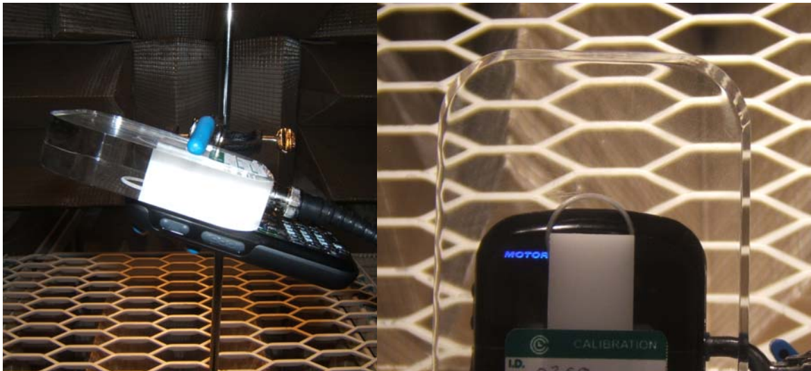
Figure 7-1 – Test holder
