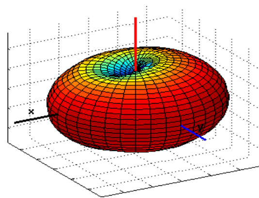
Figure 6a.6-2 Antenna pattern in the 900 MHz SMR frequency band.
