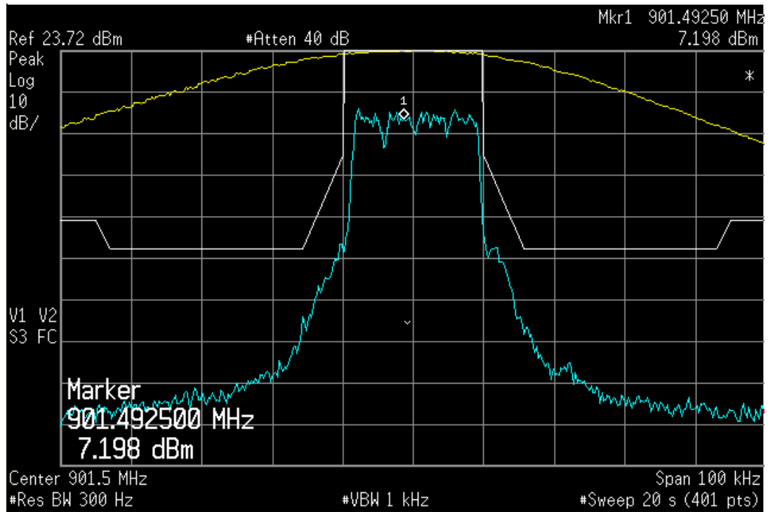
Figure 6b.2.1-2 iDEN NBPCS Band, Occupied Bandwidth, Quad-16QAM, Maximum Power.
