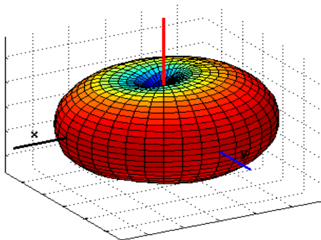
Figure 6a.6-5 Antenna pattern in the 900 MHz NBPCS frequency band.
