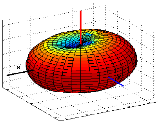
Figure 6a.6-1 Antenna pattern in the 800 MHz SMR frequency band.
