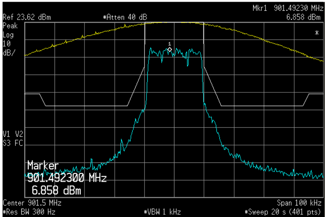
Figure 6b.2.1-1 iDEN NBPCS Band, Occupied Bandwidth, Quad-QPSK, Maximum Power.
