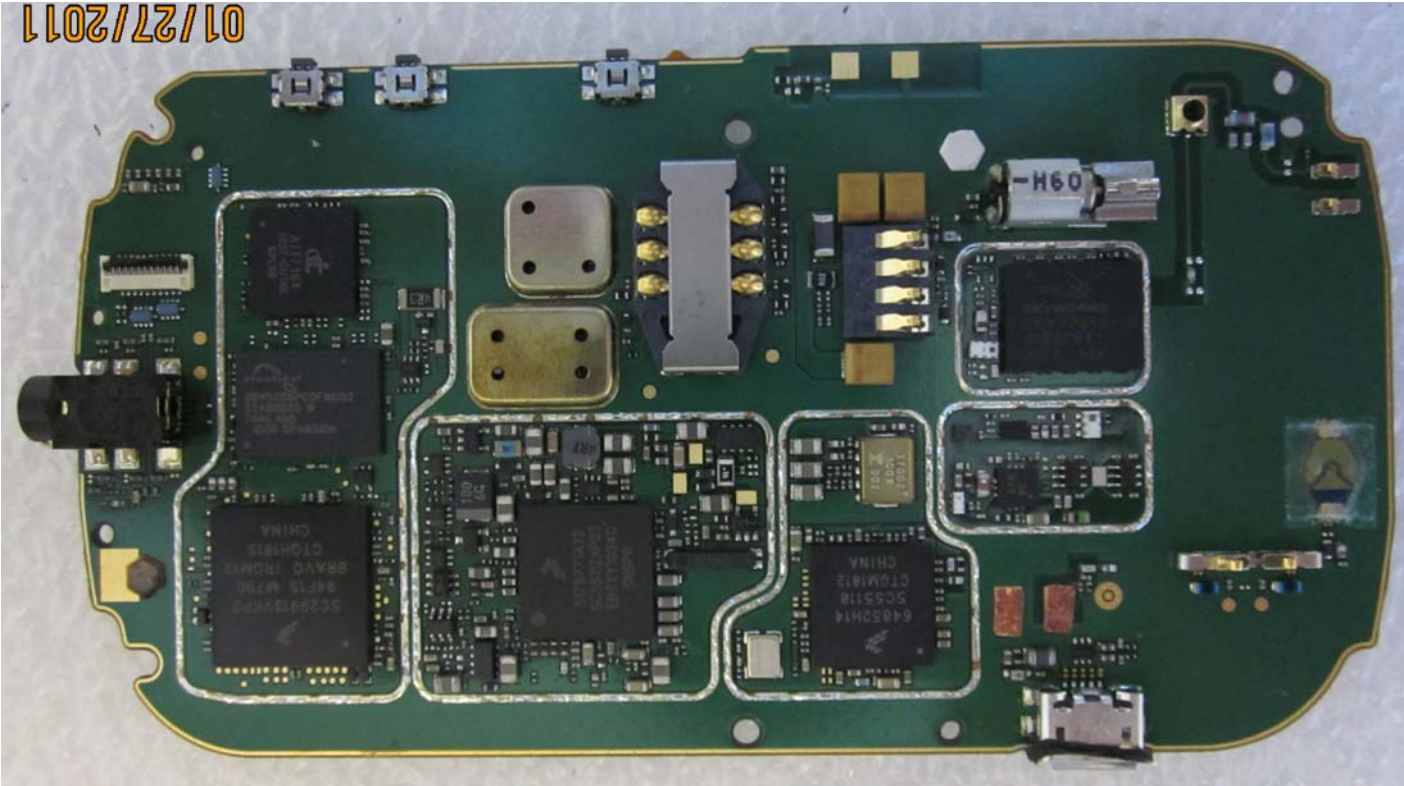
Photograph 9-2: Component side view of radio product PC Board (Shields Removed).
