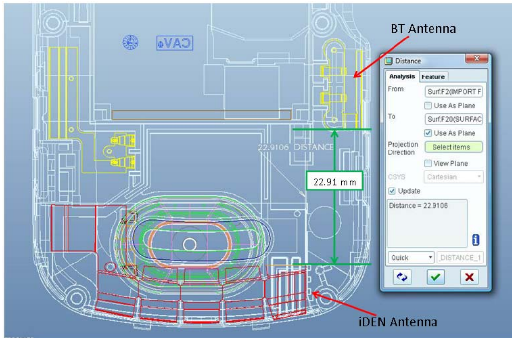
Figure 7: Antenna Separation Distances
