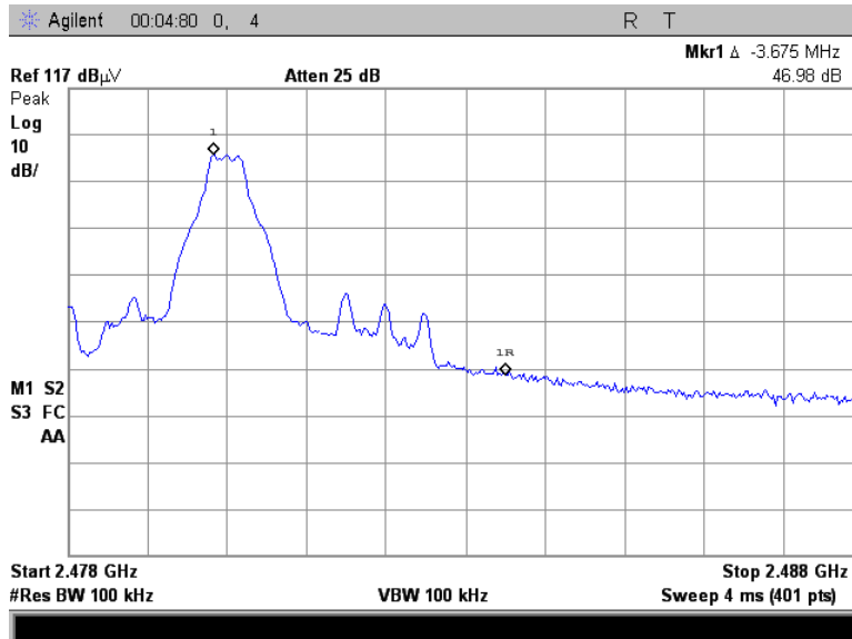
Figure 7.3.2-3: Upper Band-edge - Horizontal
