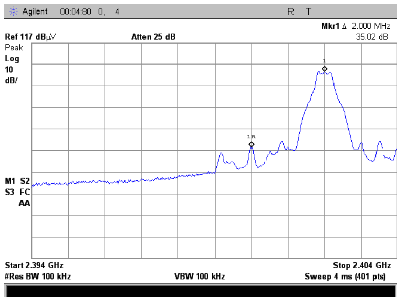
Figure 7.3.2-1: Lower Band-edge - Horizontal
