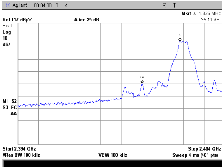
Figure 7.3.2-2: Lower Band-edge - Vertical
