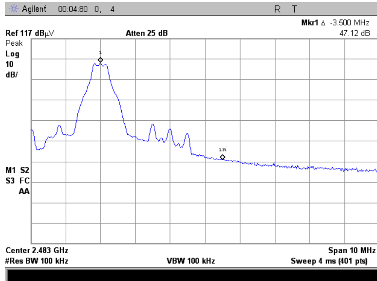
Figure 7.3.2-4: Upper Band-edge – Vertical
