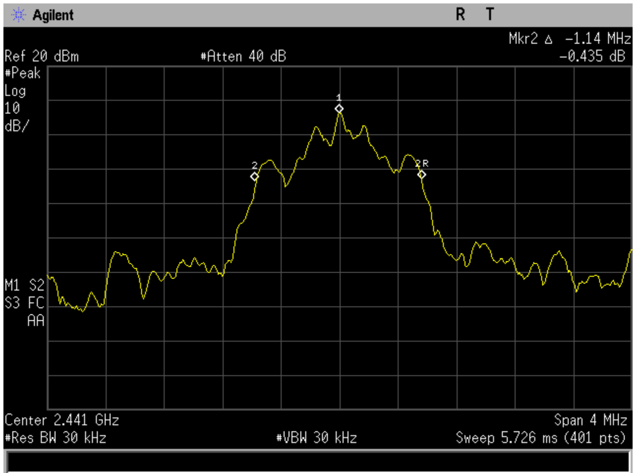
Figure 6c.2-3: Plot of 20 dB bandwidth (8-DPSK Modulation)
