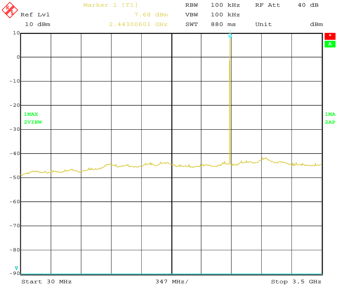
Figure 6c.7-1: Plot of spurious conducted emissions 30 MHz – 3.5 GHz.
