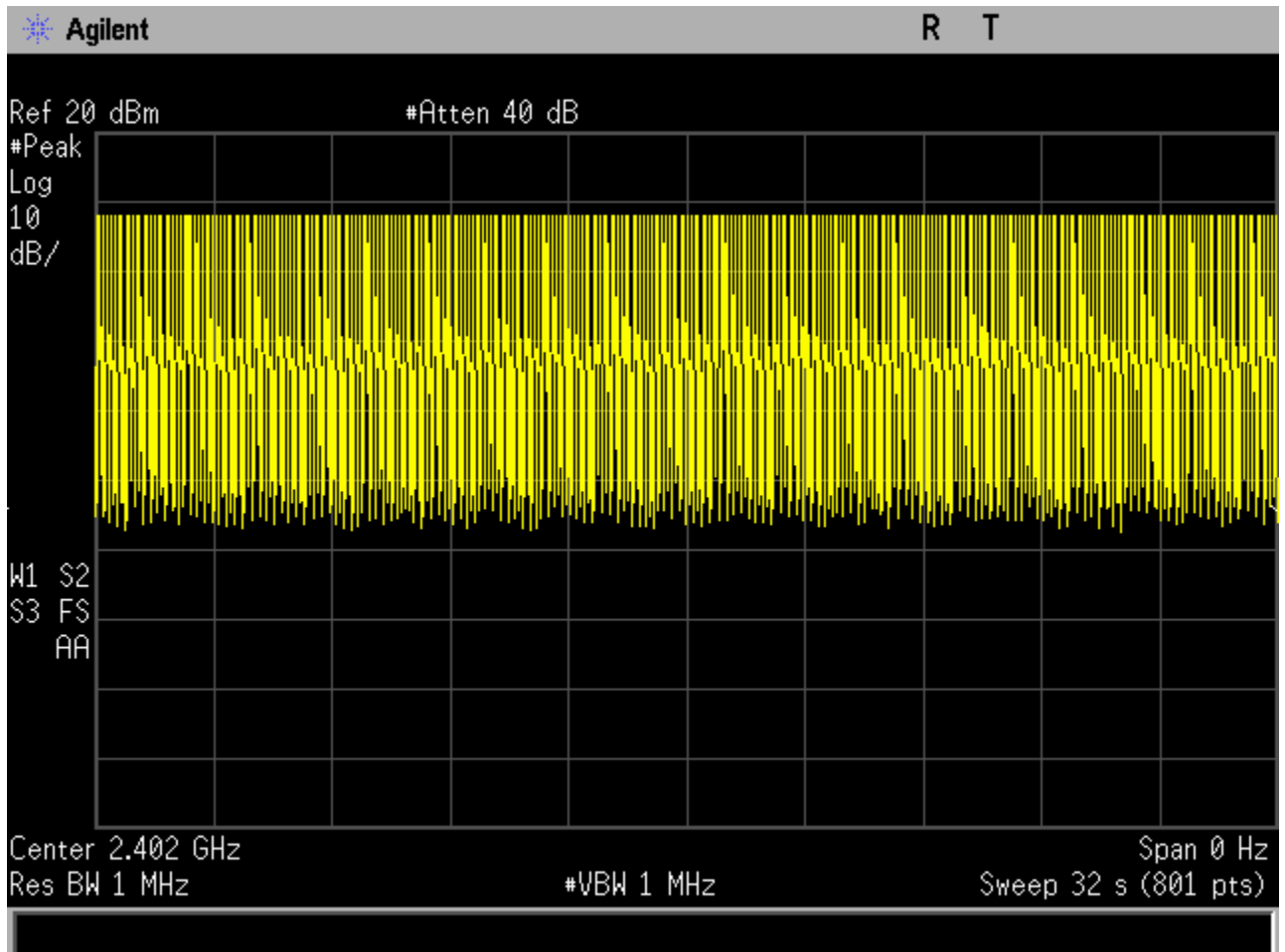
Figure 6c.4-1: Plot of dwell time over 32 second period
