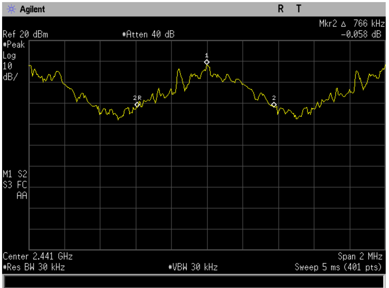
Figure 6c.2-1: Plot of 20 dB bandwidth (GFSK Modulation)
