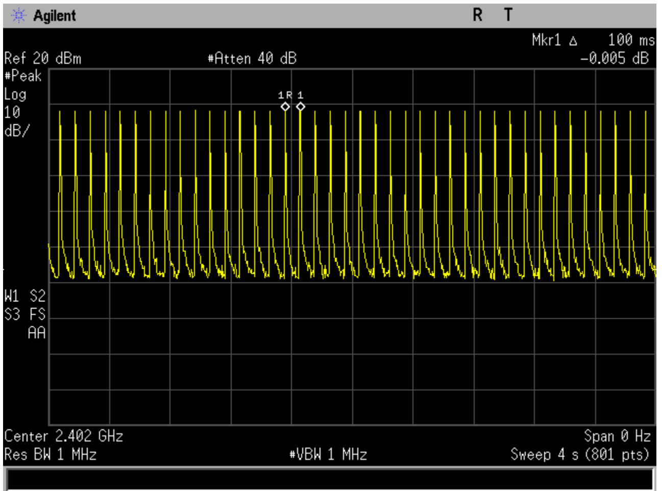
Figure 6c.4-2: Plot of dwell time over 4 second period.
