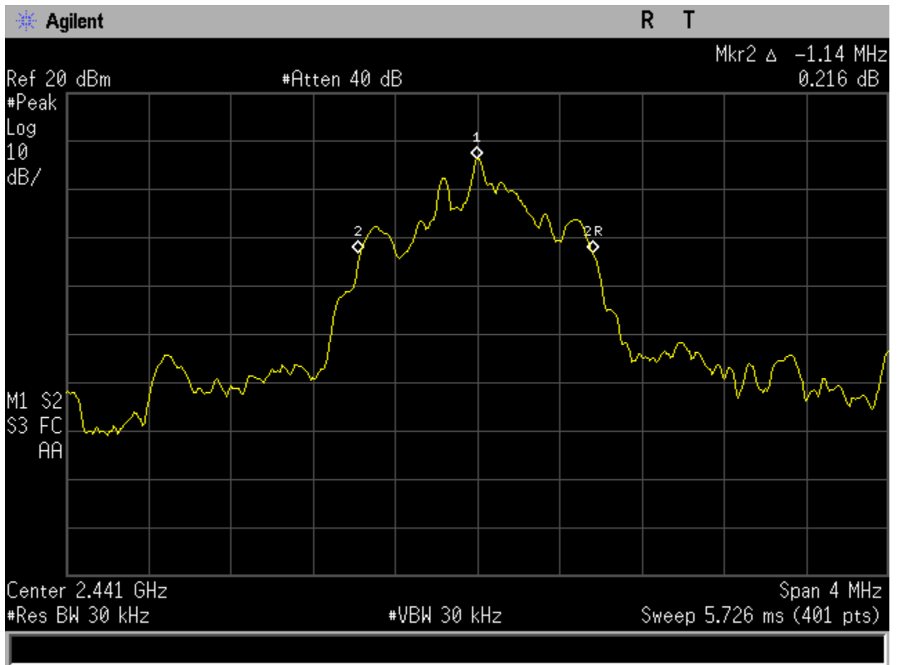
Figure 6c.2-2: Plot of 20 dB bandwidth (P/4 DPSK Modulation)
