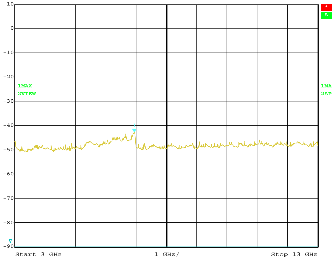
Figure 6c.7-2: Plot of spurious conducted emissions 3 GHz – 13 GHz.
