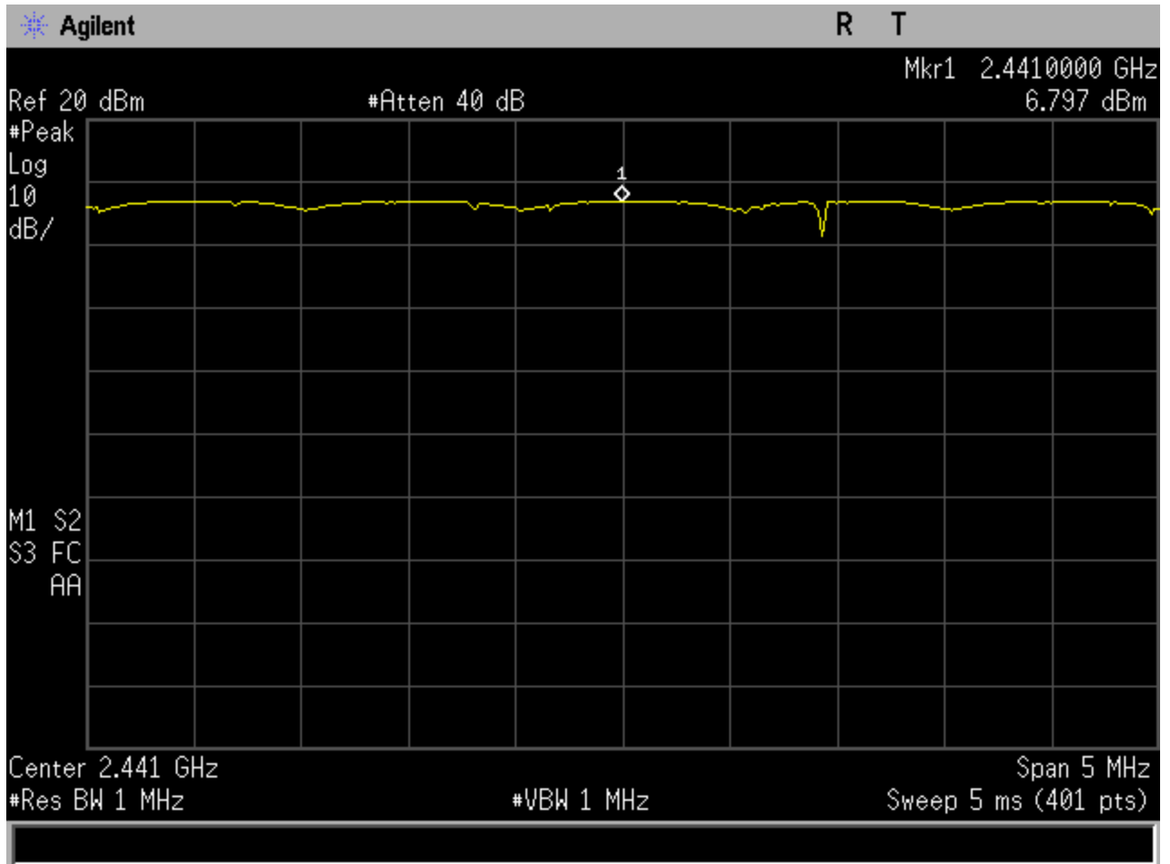
Figure 6c.5-1: Plot of peak output power
