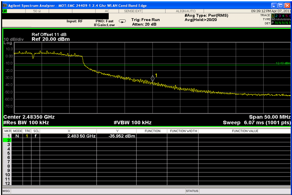
Channel 11 @ 13Mbps – Upper Band Edge
