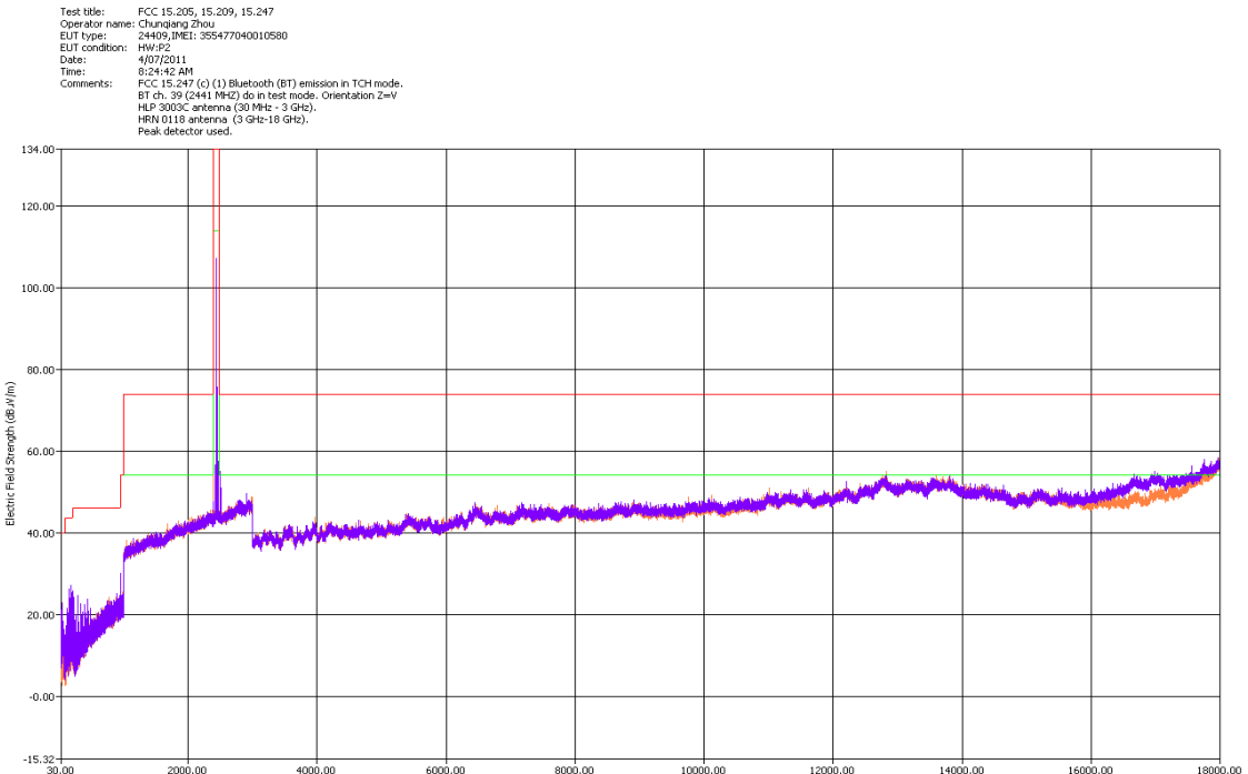
30 MHz – 18 GHz Middle Channel Dual Polarization Z –slider close
