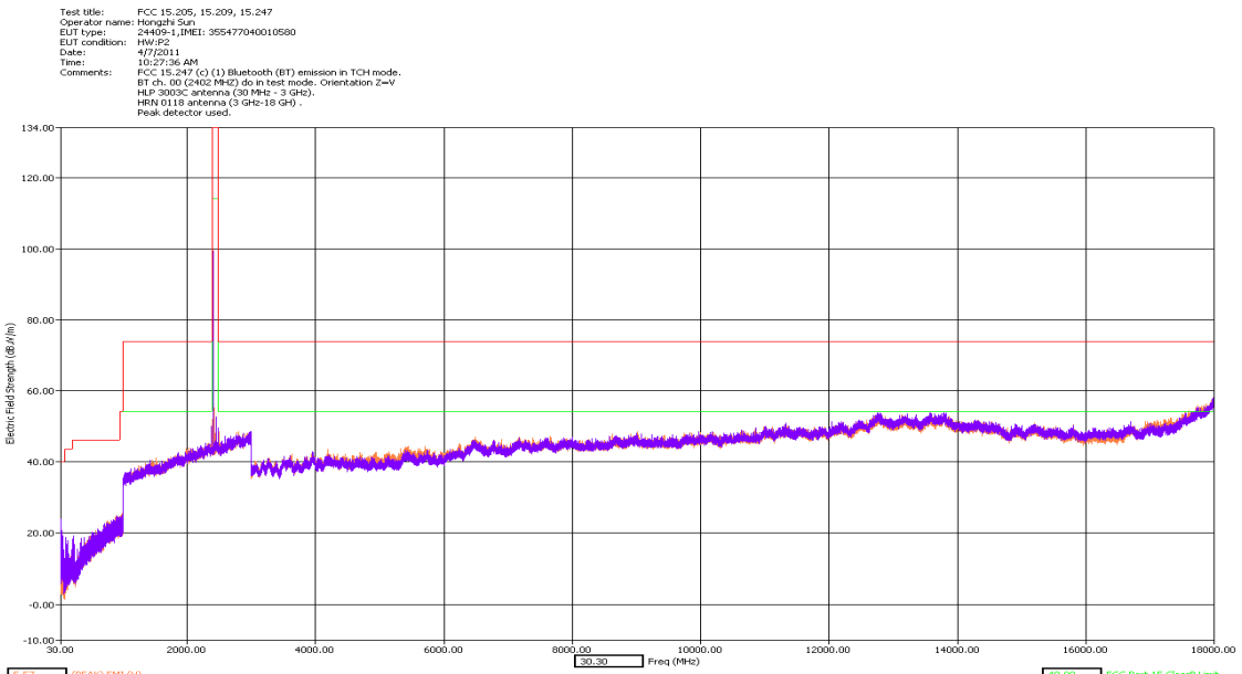
30 MHz – 18 GHz Low Channel Dual Polarization Z - slider open
