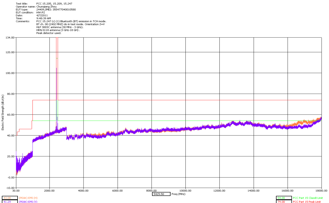
30 MHz – 18 GHz Low Channel Dual Polarization Z –slider close
