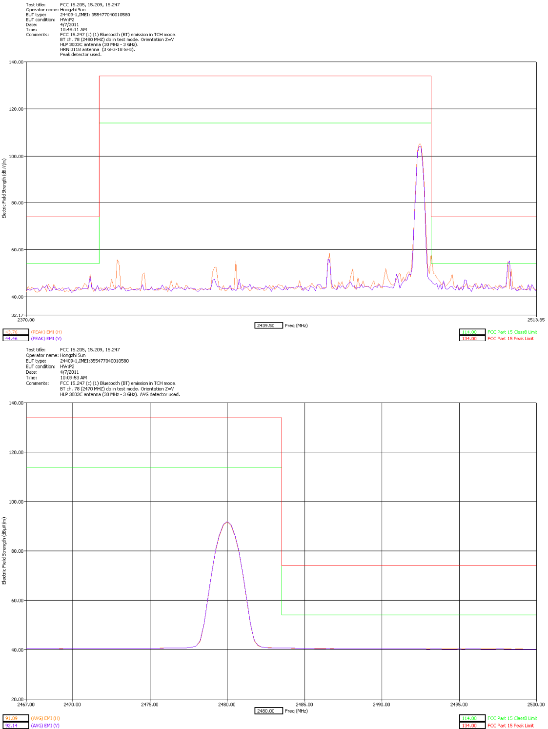
Authorized Band Emissions High Channel Dual Polarization Z - slider open
