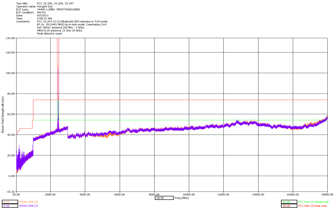
30 MHz – 18 GHz Middle Channel Dual Polarization Z - slider open
