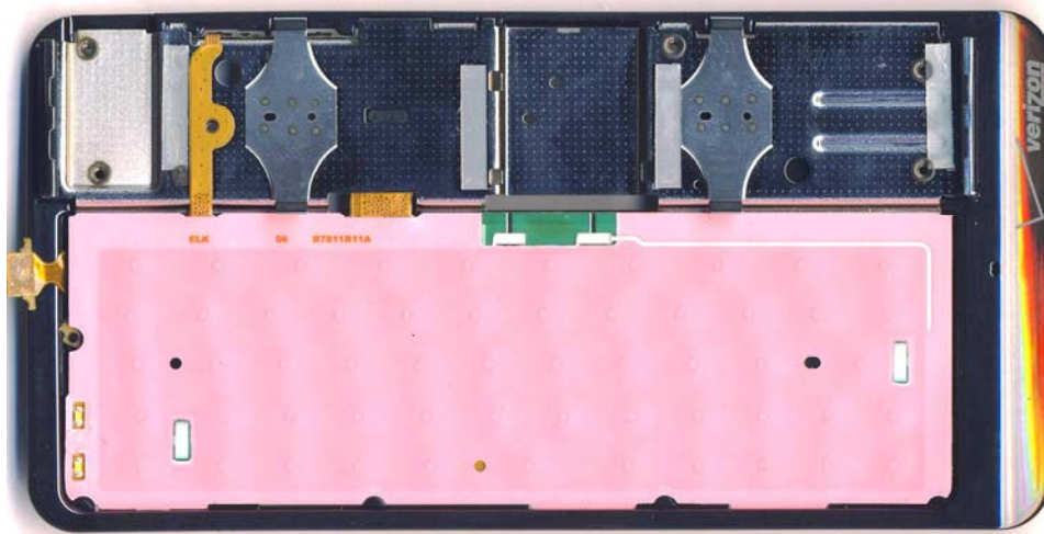
Base Assembly – Keypad Removed
