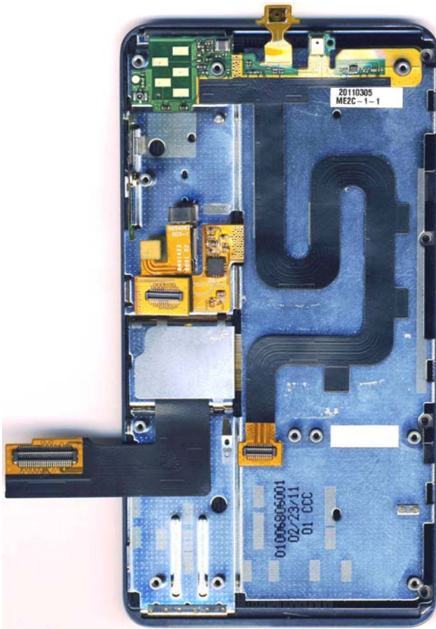
Rear Housing and Main Board Removed
