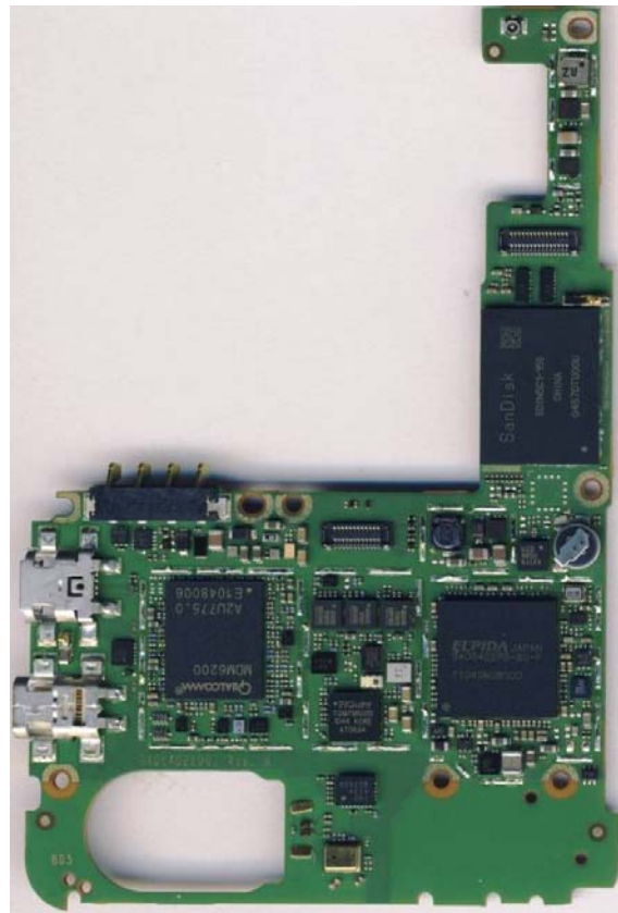
Main Board Top without Shields
