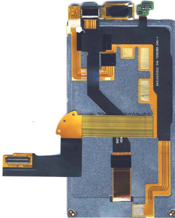
Display Slide Assembly Front
