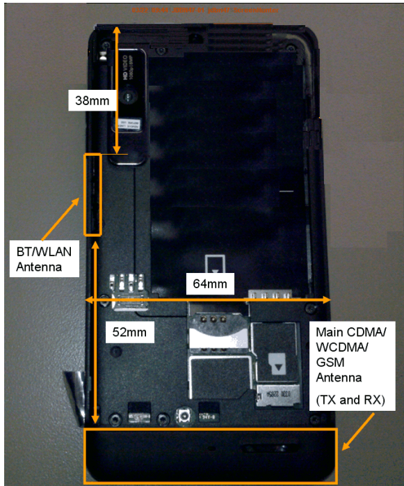
Closest distance between CDMA antenna and BT/WIFI antenna is 5.2 cm
