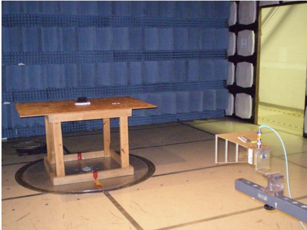
Tx Radiated
