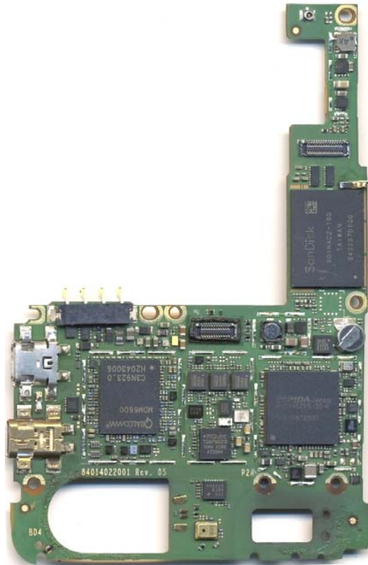
Main Board Top Without Shields
