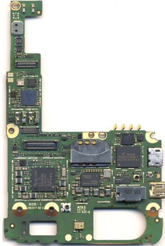
Main Board Bottom Without Shield
