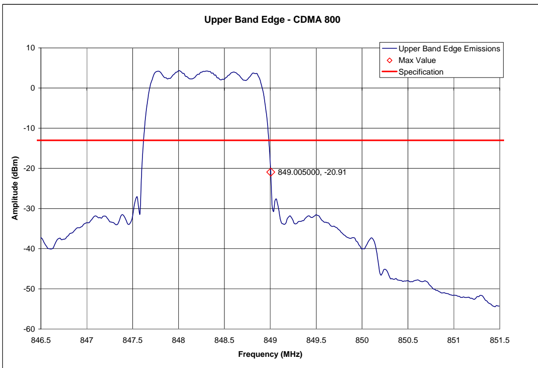
CDMA 800 – Upper Band Edge – Channel 777 (848.31MHz)
