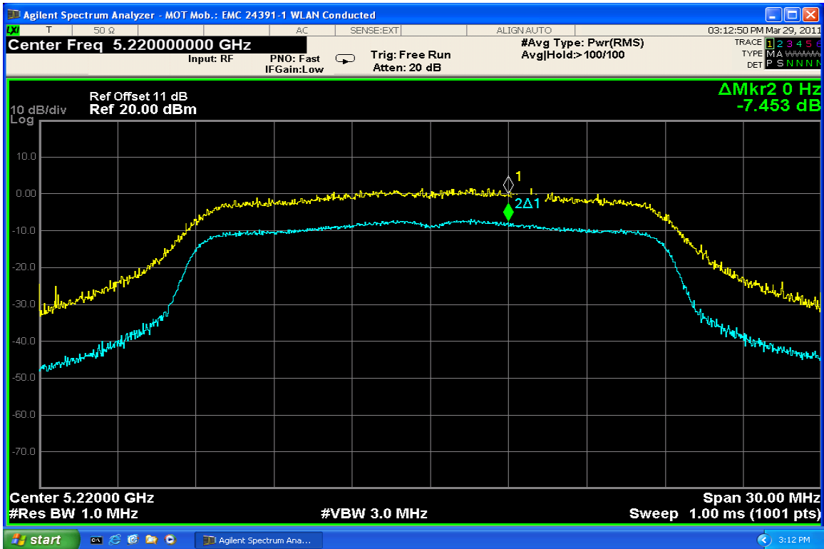
Peak Excursion Ch. 44 @ 14.4Mbps
