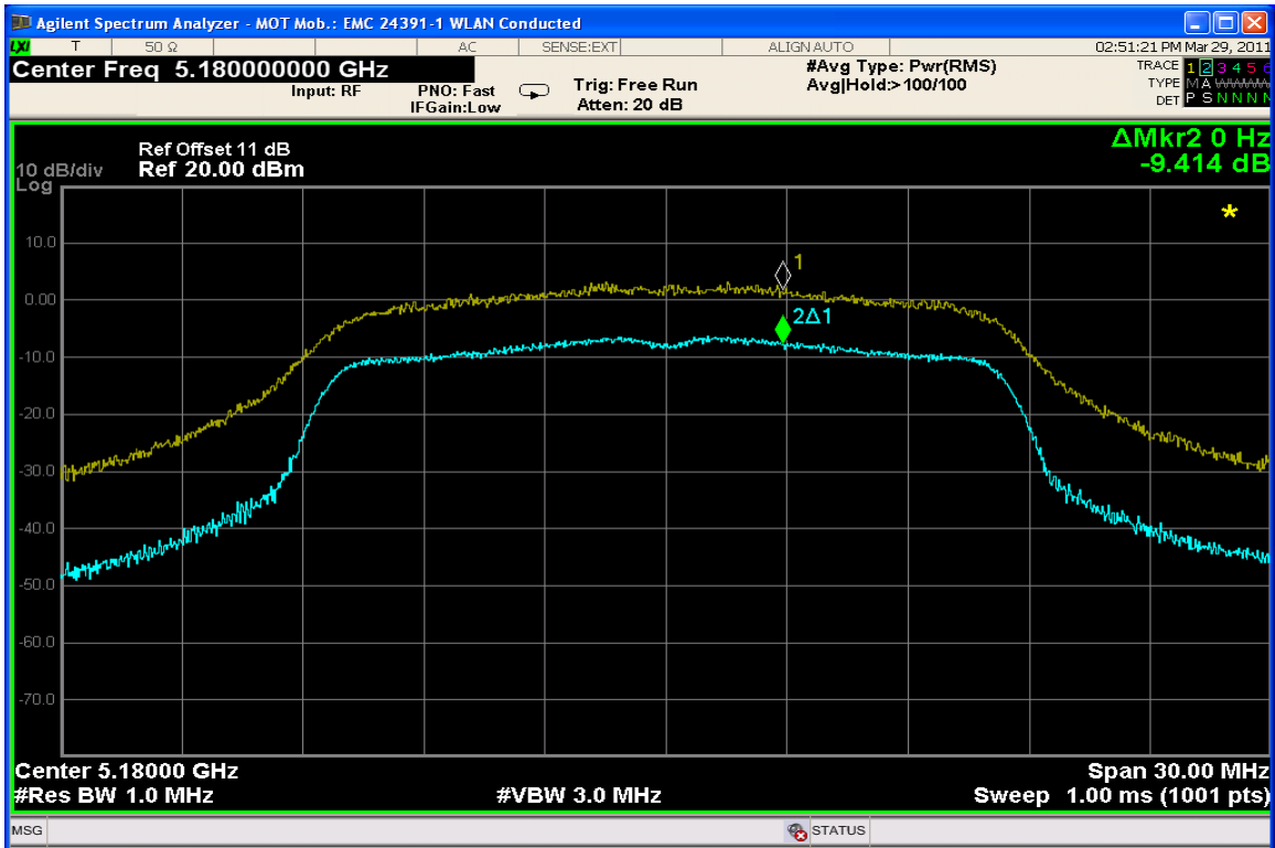
Peak Excursion Ch. 36 @ 12Mbps
