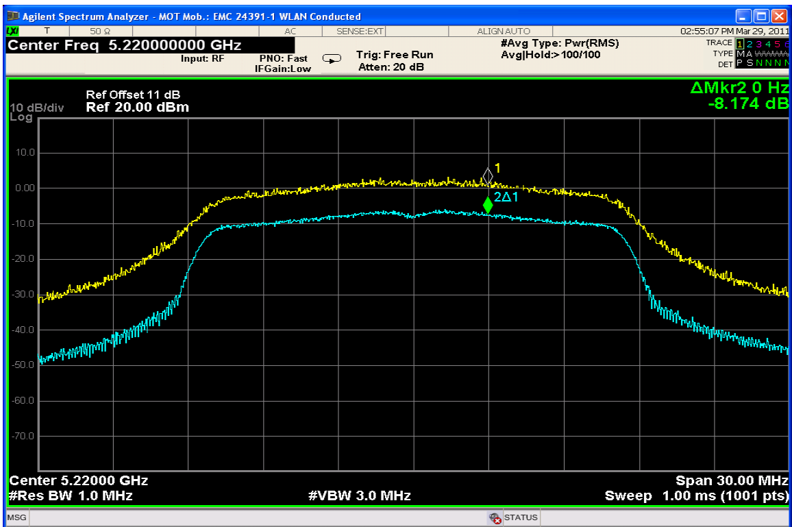
Peak Excursion Ch. 44 @ 12Mbps
