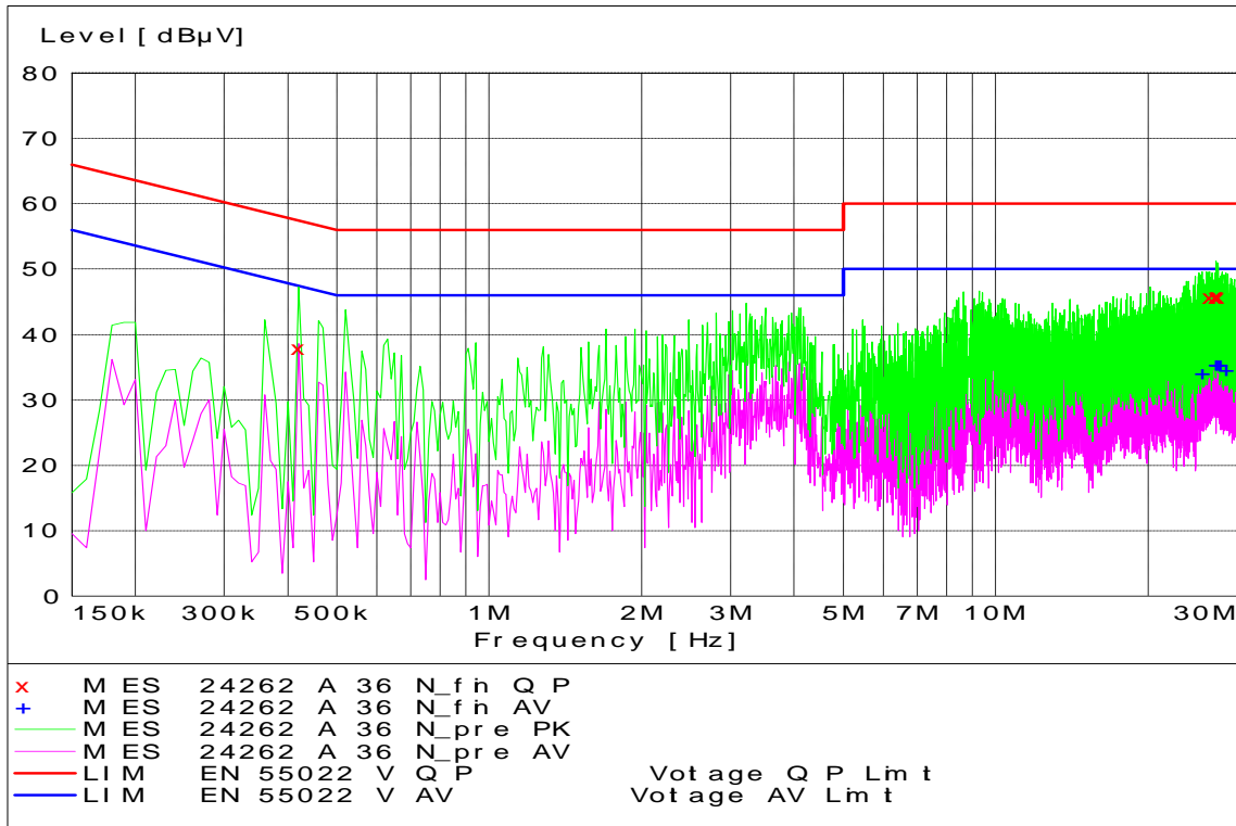
WLAN Channel 36 - Tx Mode - Neutral Coupling
