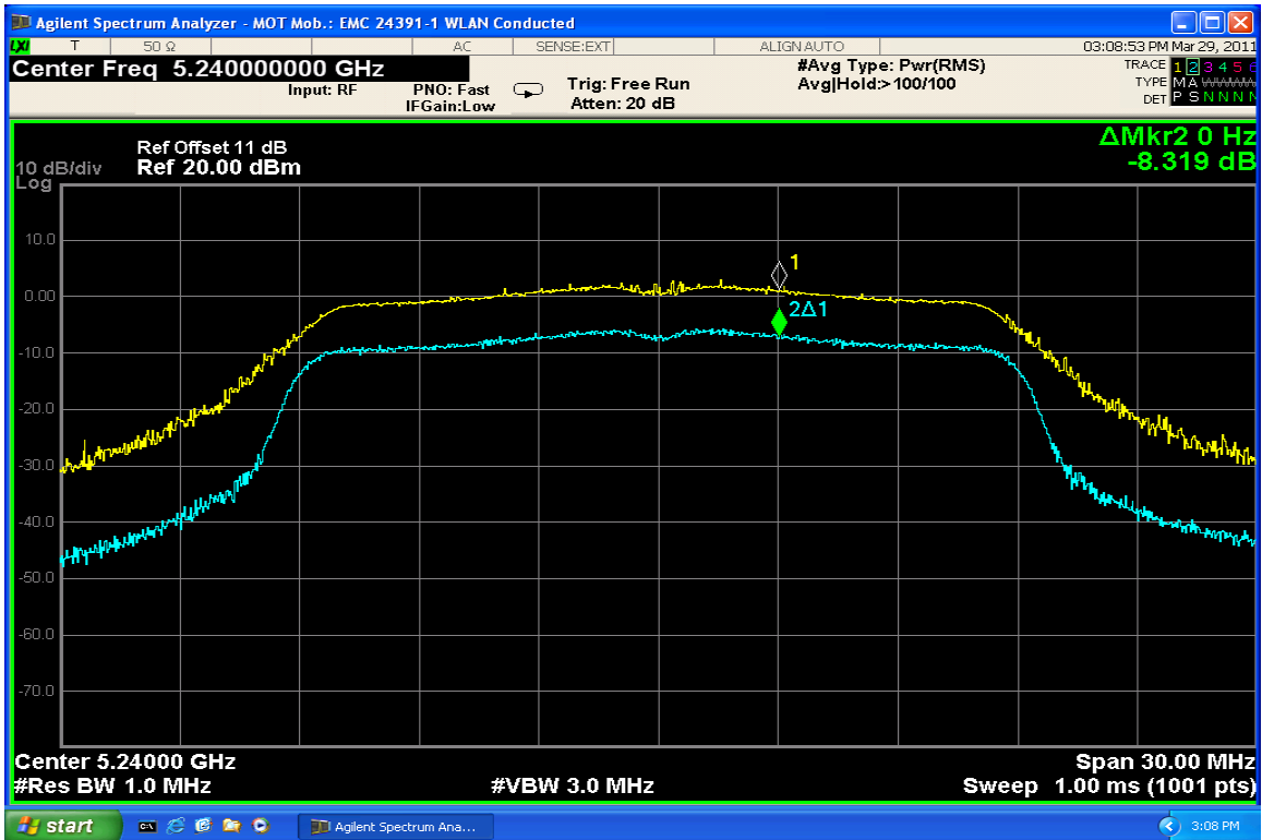
Peak Excursion Ch. 48 @ 6.5Mbps
