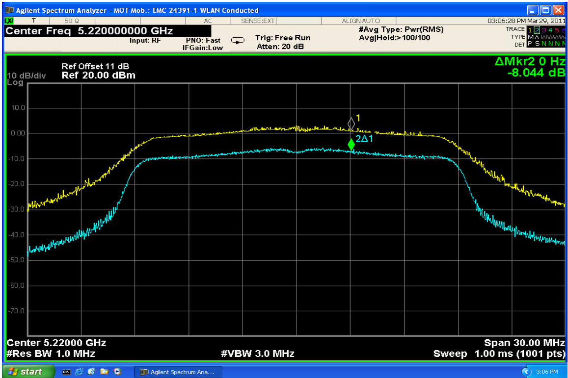
Peak Excursion Ch. 44 @ 6.5Mbps
