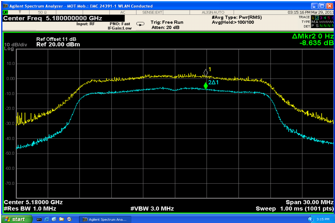
Peak Excursion Ch. 36 @ 14.4Mbps
