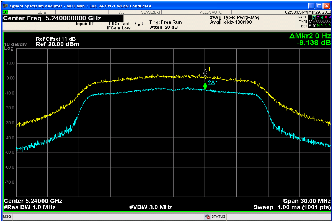
Peak Excursion Ch. 48 @ 12Mbps
