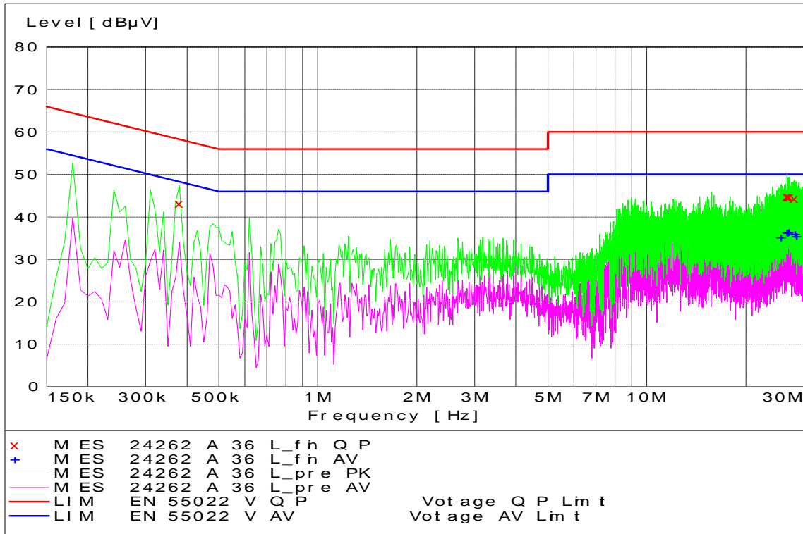
WLAN Channel 36 - Tx Mode - Line Coupling
