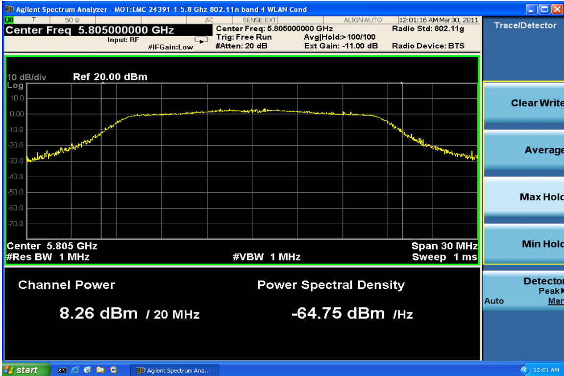
Max. Power Channel 161 @ 6.5 Mbps 802.11 n @ 7.2 Mbps
