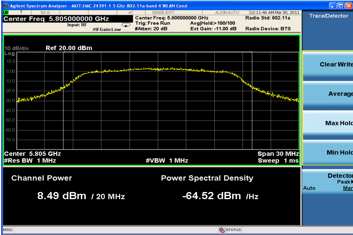
Max. Power Channel 161 @ 12 Mbps
