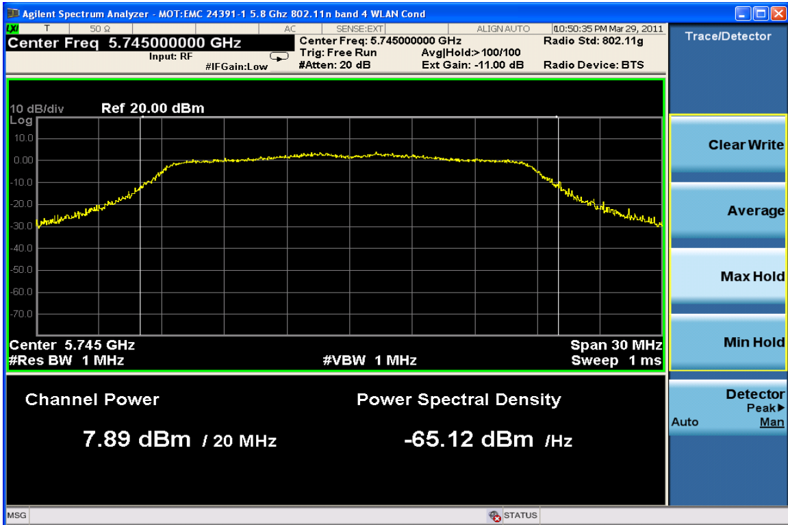
Max. Power Channel 149 @ 7.2 Mbps
