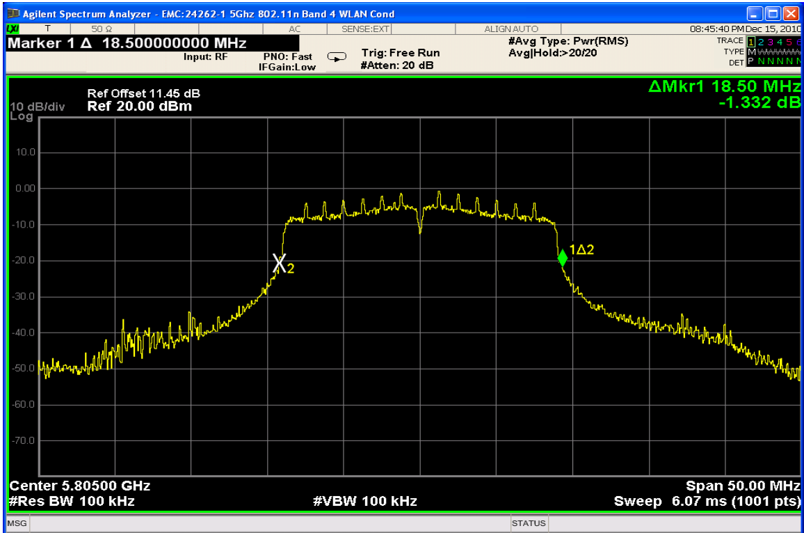
20 dB Bandwidth Channel 161 @ 7.2 Mbps
