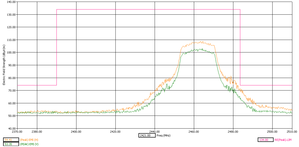
High Band Edge X Orientation Peak Detector
