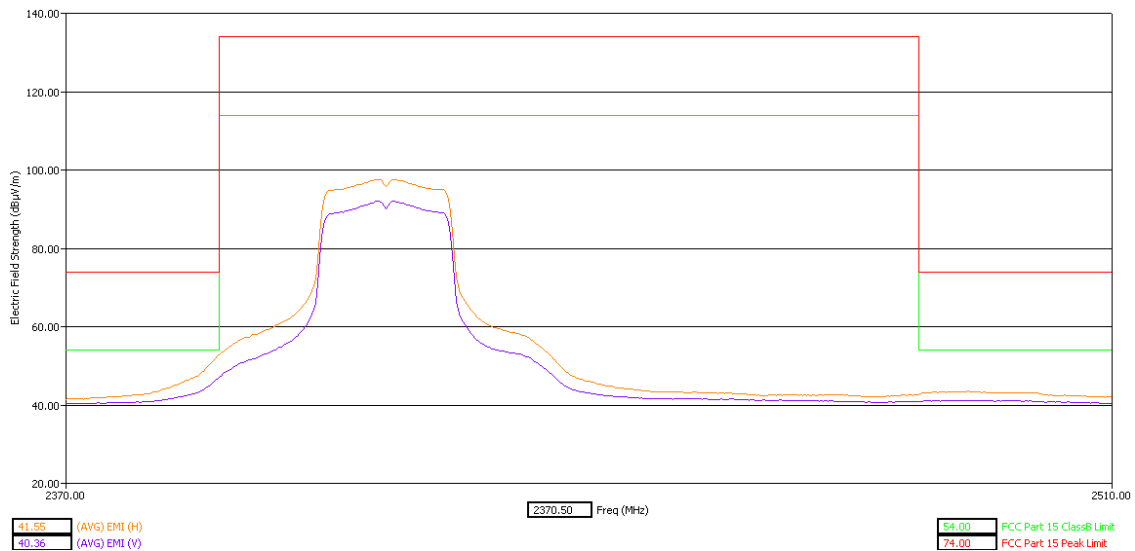
Low Band Edge X Orientation AVG Detector
