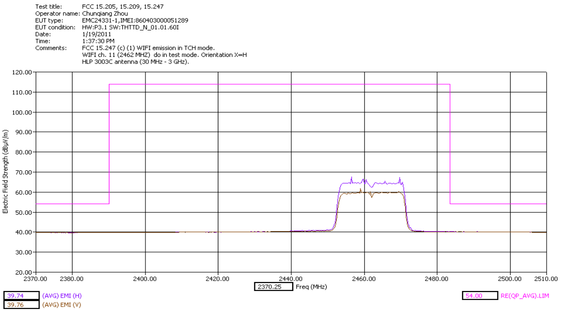
High Band Edge X Orientation AVG Detector
