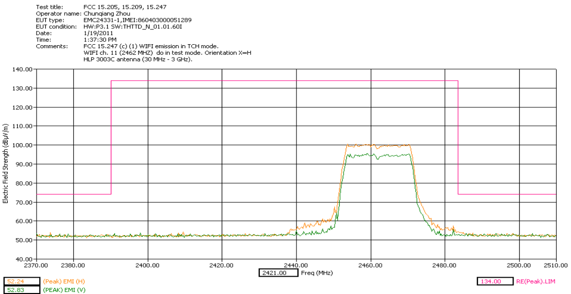
High Band Edge X Orientation Peak Detector
