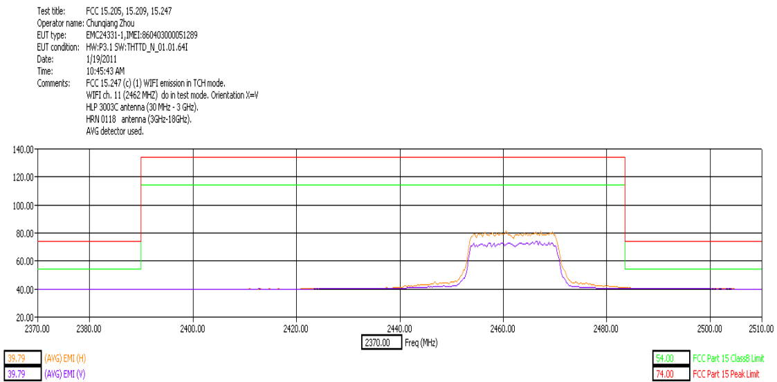
High Band Edge X Orientation AVG Detector
