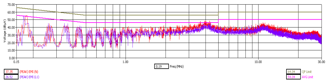
WLAN Channel 6 - Tx Mode - Peak Detector
