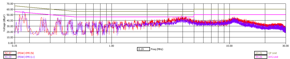
WLAN Channel 1 - Tx Mode -Peak Detector
