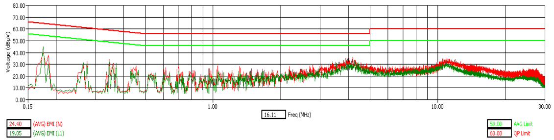
WLAN Channel 1 - Tx Mode - AVG Detector
