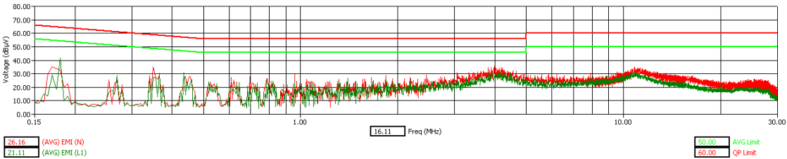
WLAN Channel 11 - Tx Mode - AVG Detector
