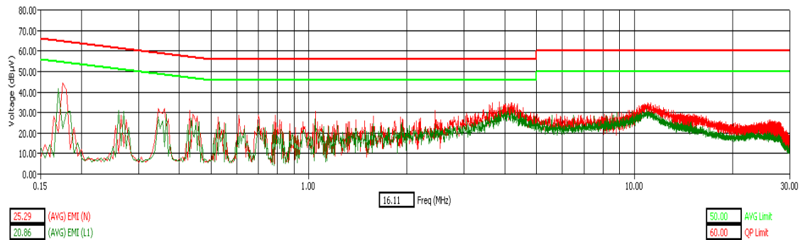
WLAN Channel 6 - Tx Mode - AVG Detector
