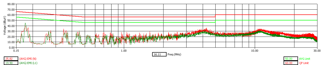
WLAN Channel 1 - Tx Mode - AVG Detector
