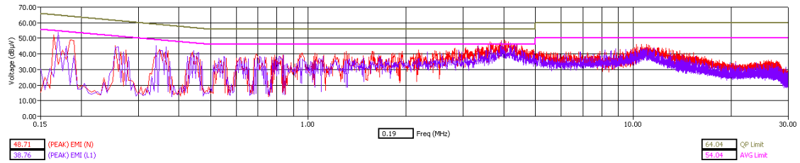
WLAN Channel 11 - Tx Mode - Peak Detector
