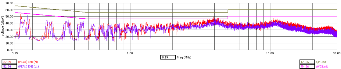
WLAN Channel 6 - Tx Mode - Peak Detector
