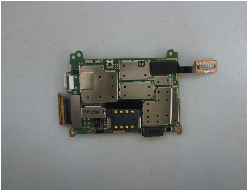
Main PCB top with shielding
