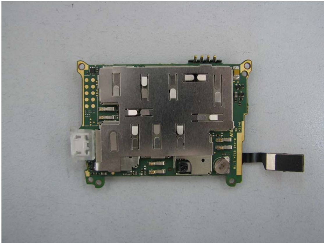
Main PCB bottom with shielding
