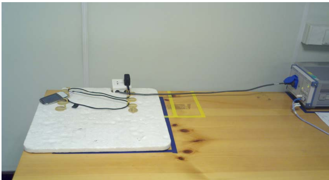
AC Line Conducted Emissions
