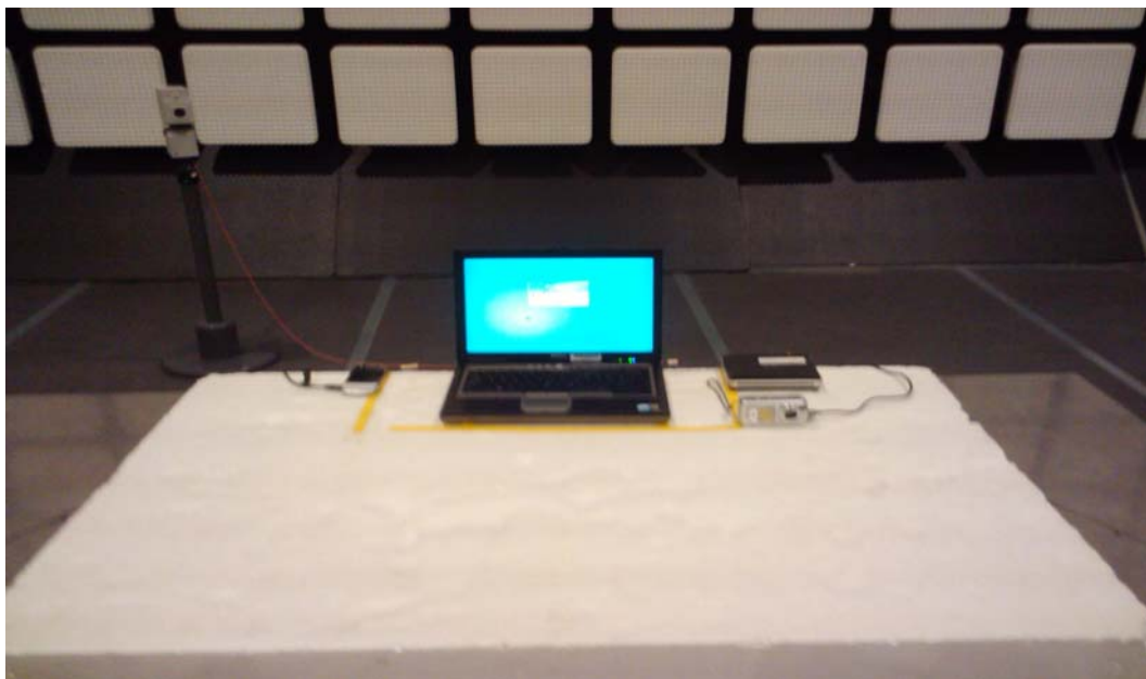
Radiated Emissions – Computer Peripheral
