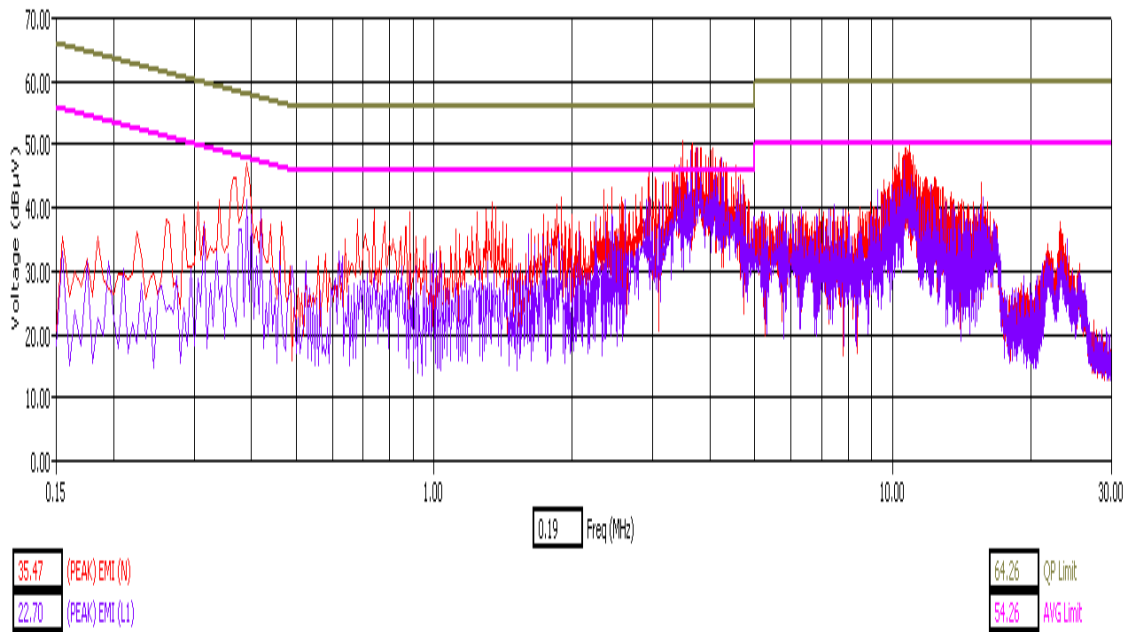
Bluetooth – Hopping - Tx Mode – Peak Detector
