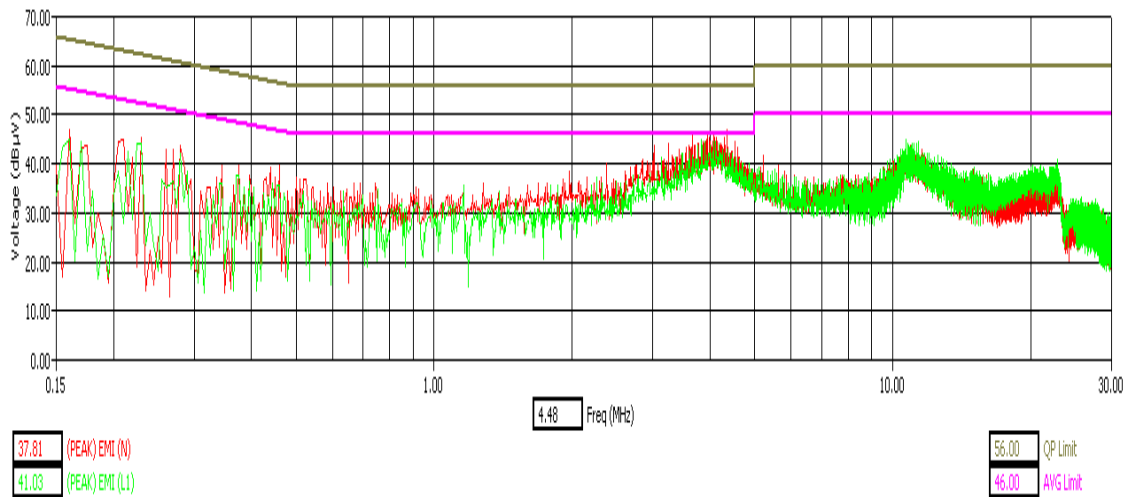
Bluetooth – Hopping - Tx Mode – Peak Detector
