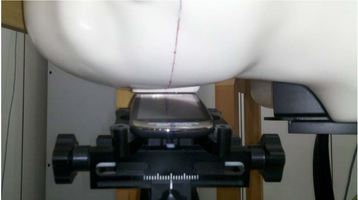
Figure 6: Tilt Position, Front of Head of Phantom
