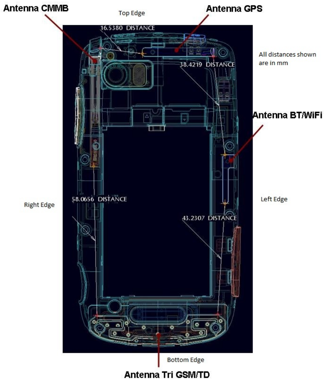
Figure 3: Antenna Separation Distances
