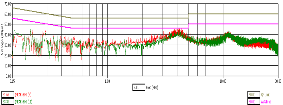
WLAN Channel 11 - Tx Mode - Peak Detector
