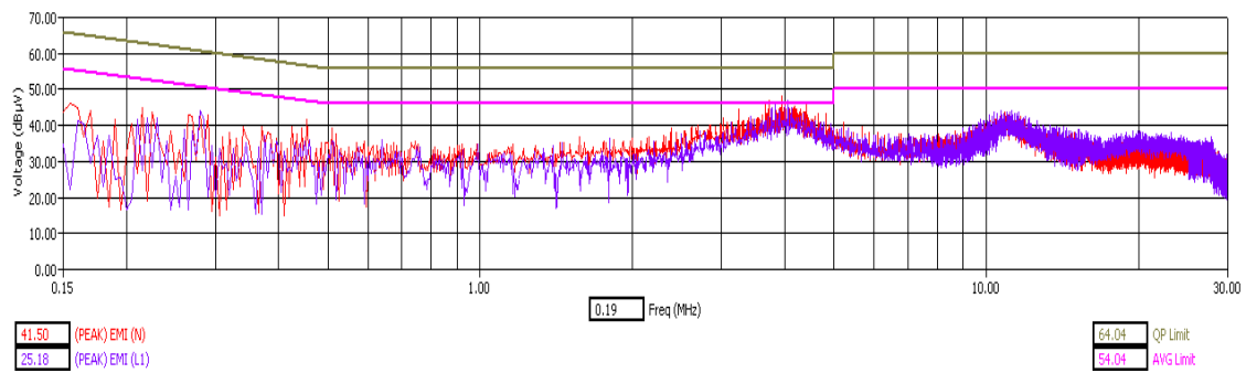
WLAN Channel 11 - Tx Mode - Peak Detector
