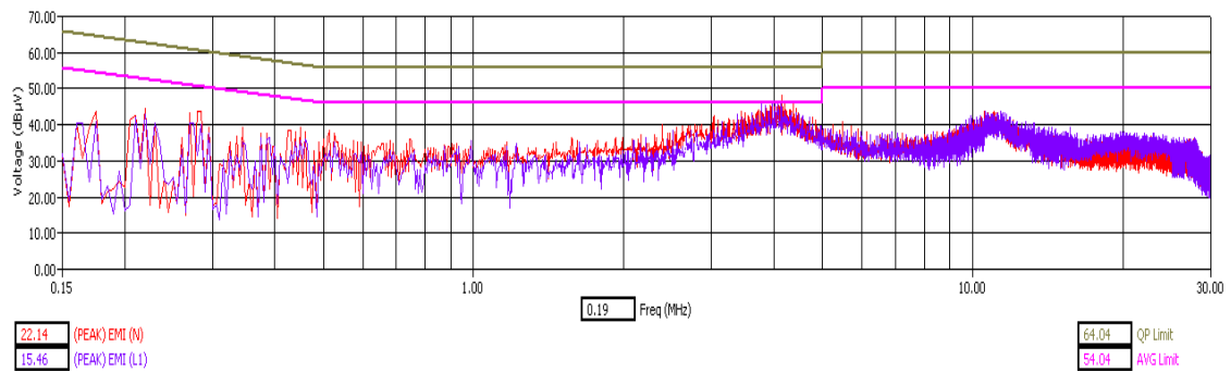
WLAN Channel 6 - Tx Mode - Peak Detector
