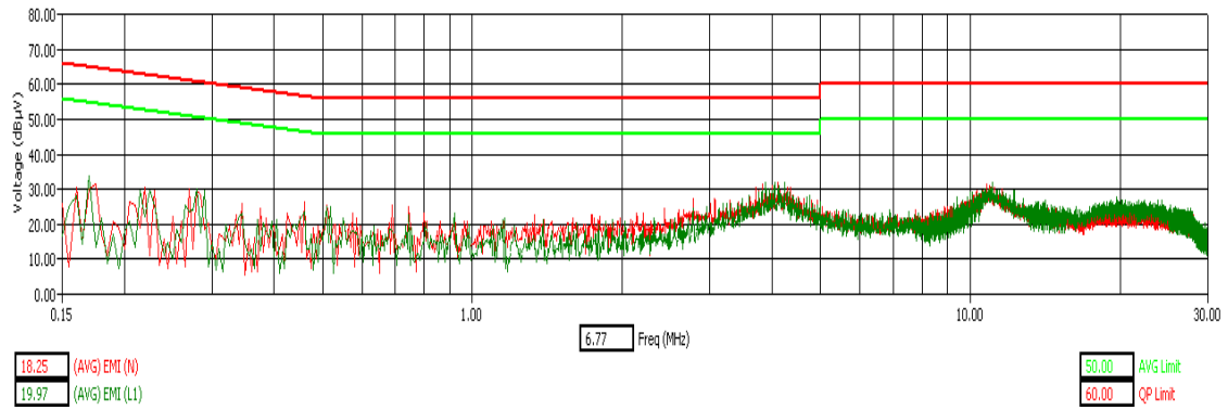
WLAN Channel 1 - Tx Mode - AVG Detector
