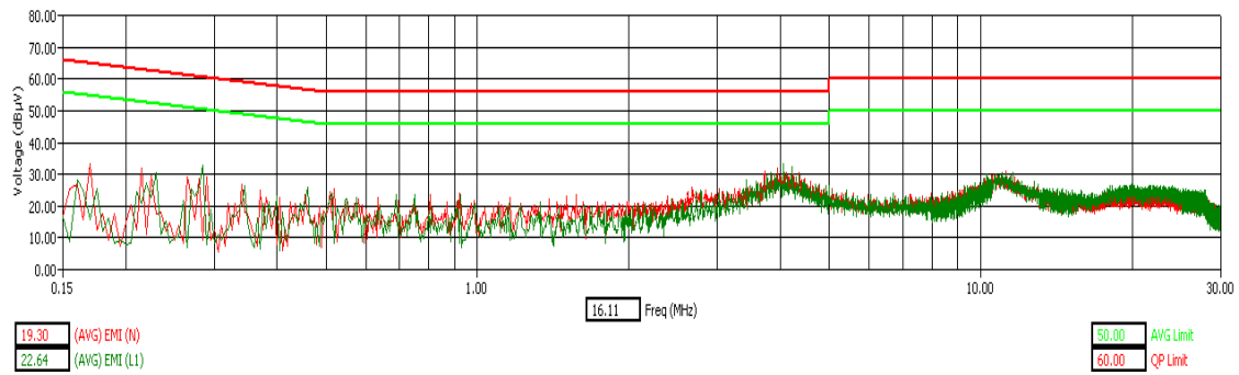
WLAN Channel 11 - Tx Mode - AVG Detector
