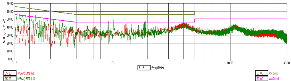
WLAN Channel 1 - Tx Mode -Peak Detector
