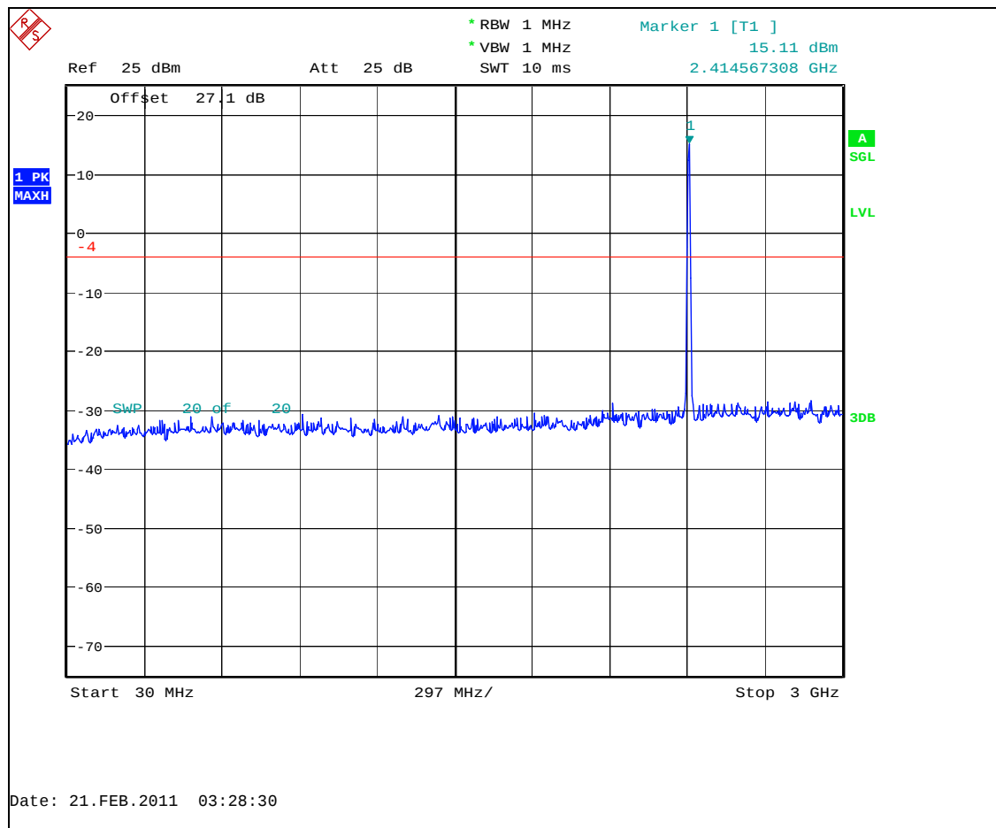
Conducted Spurious Emissions 30-3000MHz (Low Channel)
