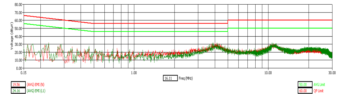
WLAN Channel 6 - Tx Mode - AVG Detector
