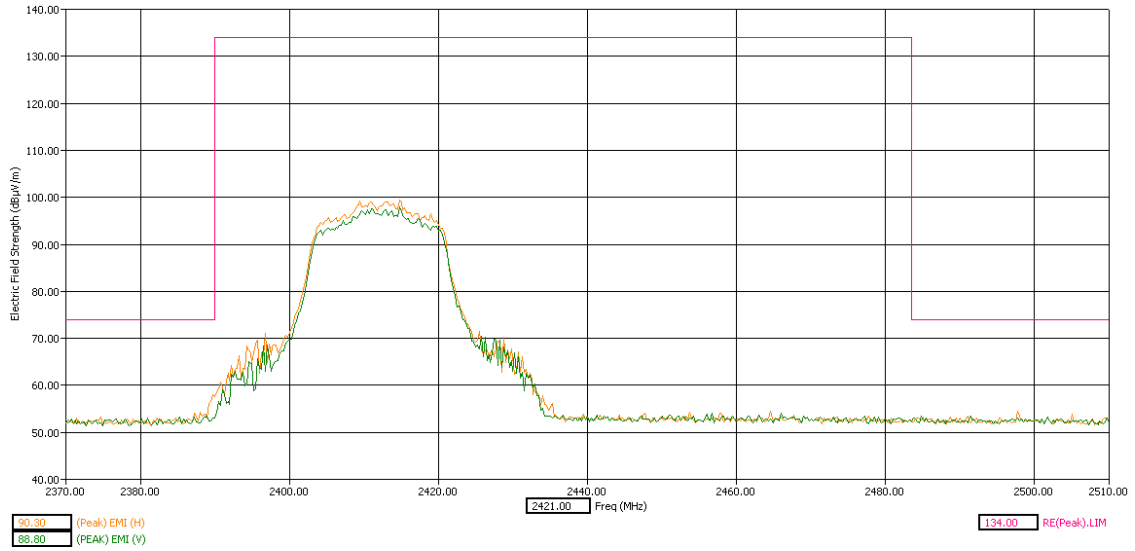
Low Band Edge Y Orientation Peak Detector
