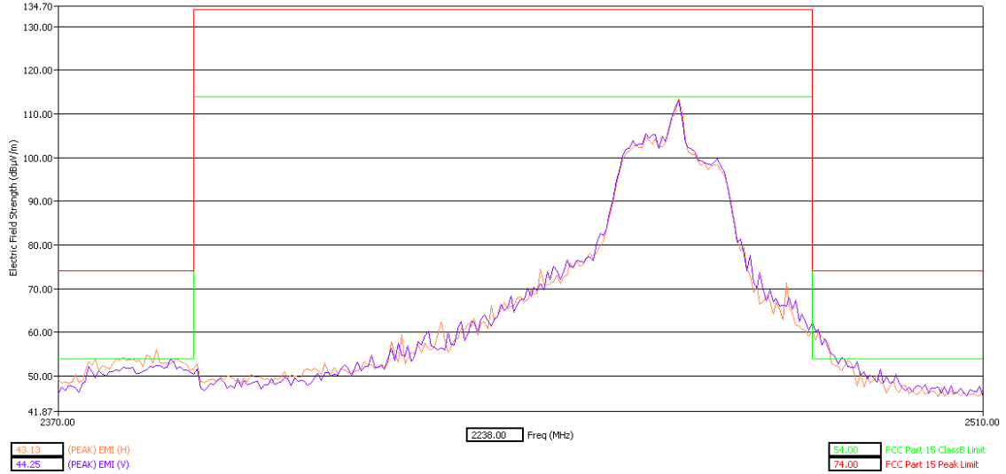
High Band Edge Y Orientation Peak Detector
