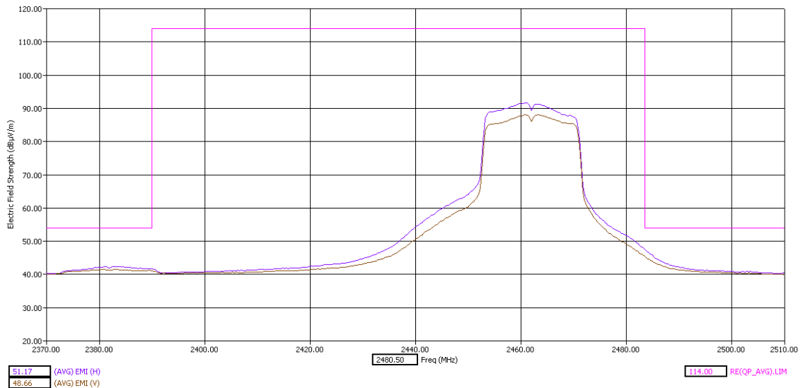
High Band Edge Y Orientation AVG Detector
