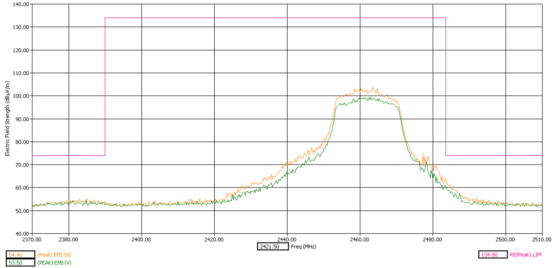
High Band Edge Y Orientation Peak Detector
