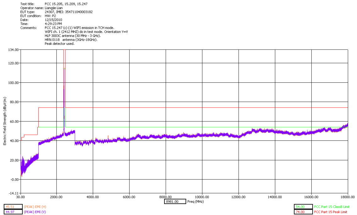
30 - 18000MHz Low Channel Dual Polarization Y
