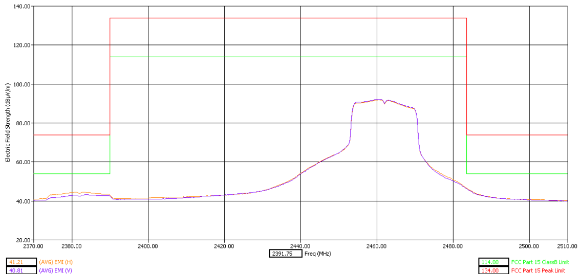
High Band Edge Y Orientation AVG Detector
