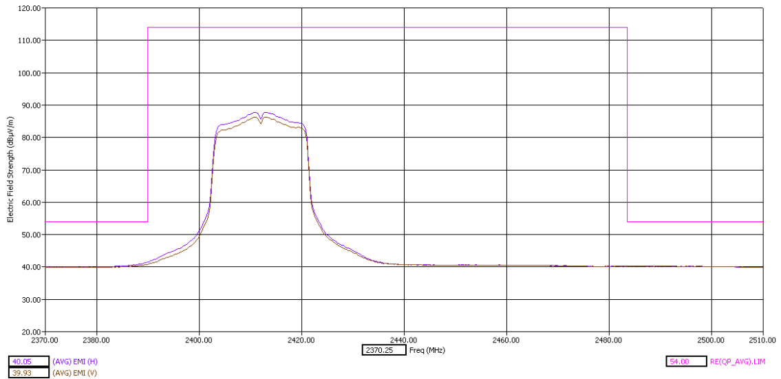
Low Band Edge Y Orientation AVG Detector
