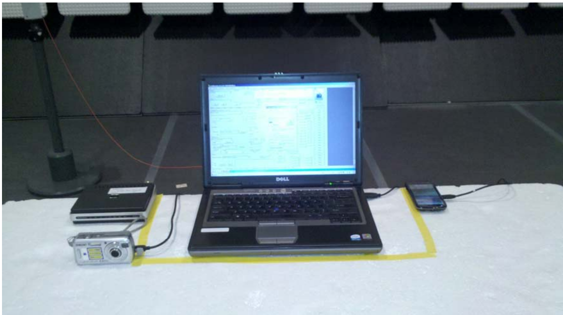
Radiated Emissions – Computer Peripheral
