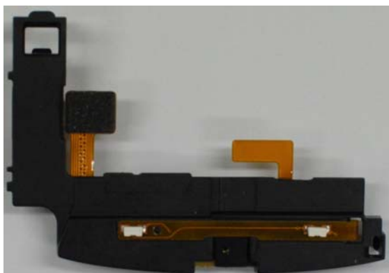
Speaker flex Top W/ Holder
