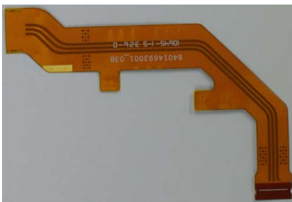
LCD Bridge flex Top
