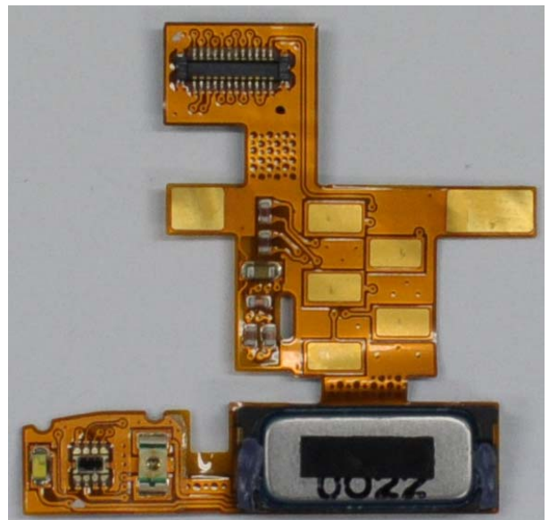
Receiver flex Bottom
