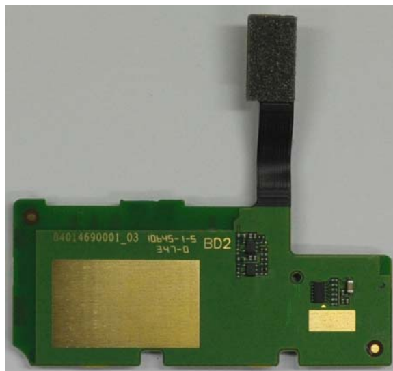
Daughter Board Top W/O Ground Plate
