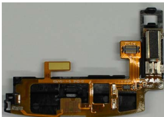
Speaker flex Top W/ Holder
