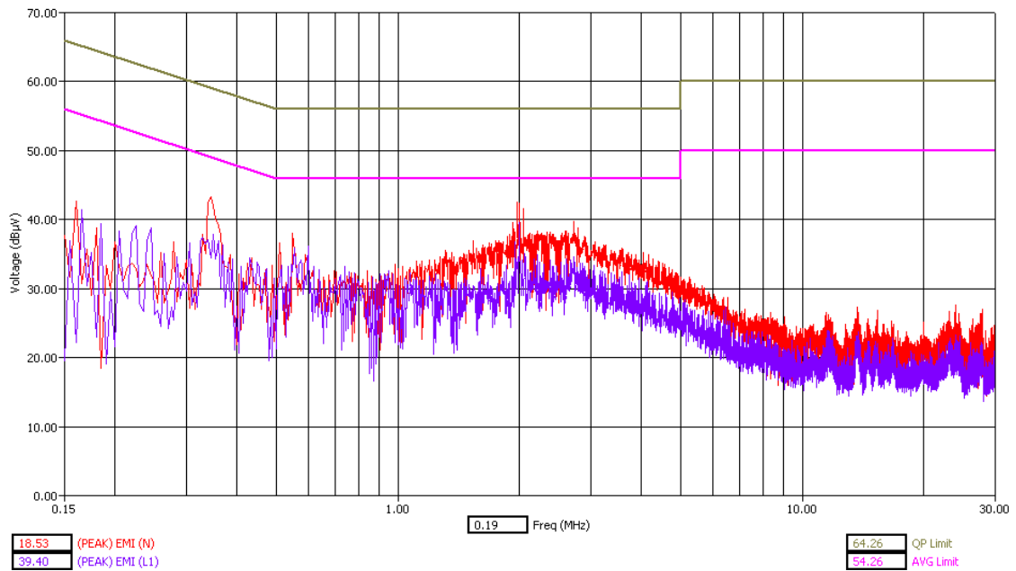
Bluetooth - Hopping - Tx Mode - Peak Detector
