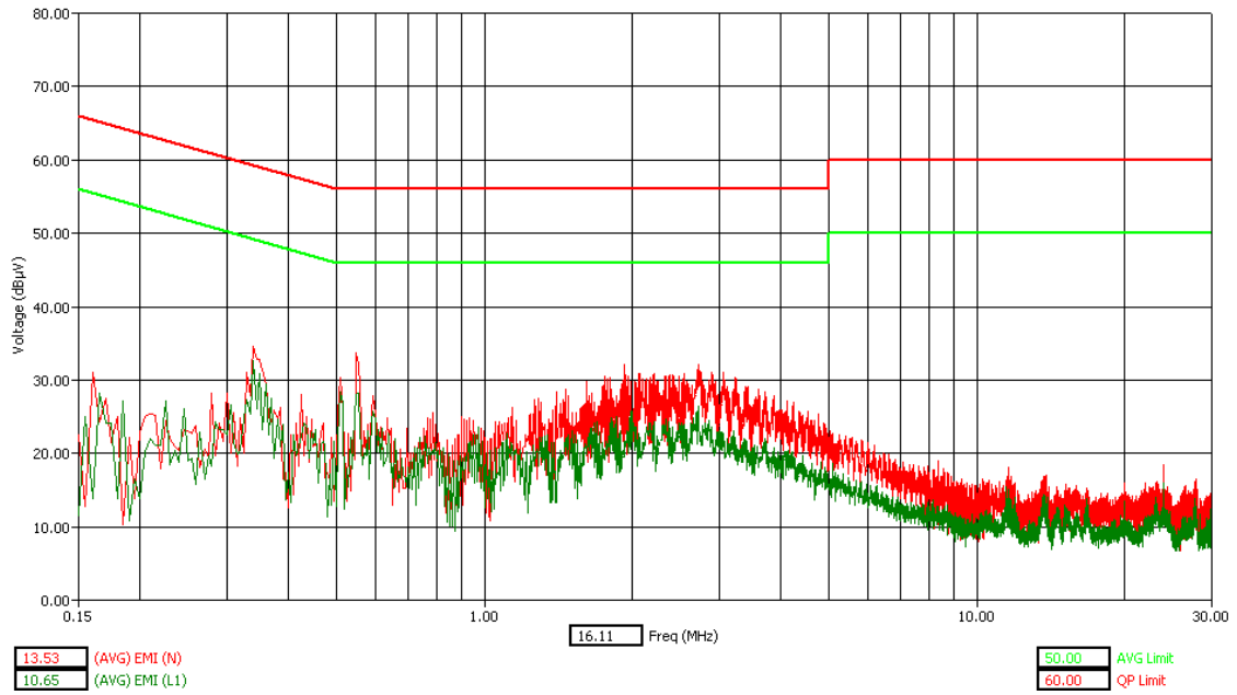
Bluetooth - Hopping - Tx Mode - AVG Detector
