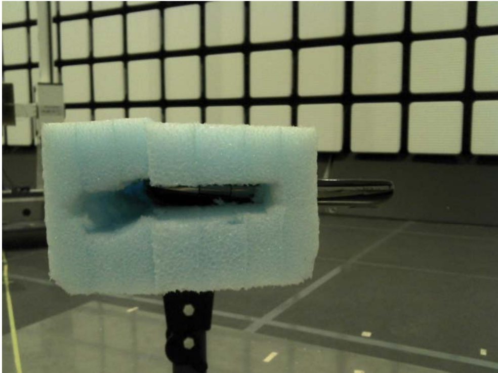
BT & WLAN X Position
