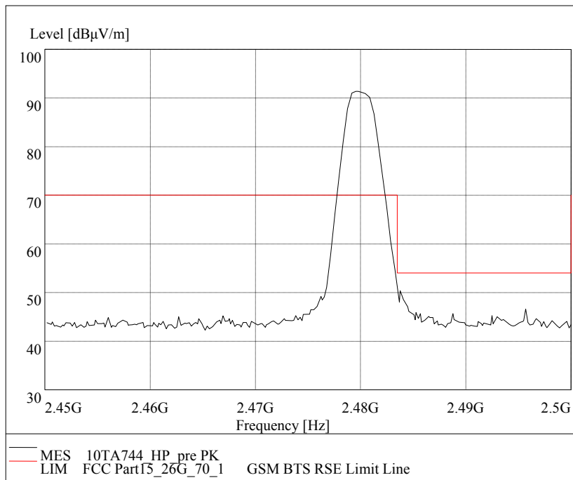
Fig.23 Radiated emission (Power): GFSK,
