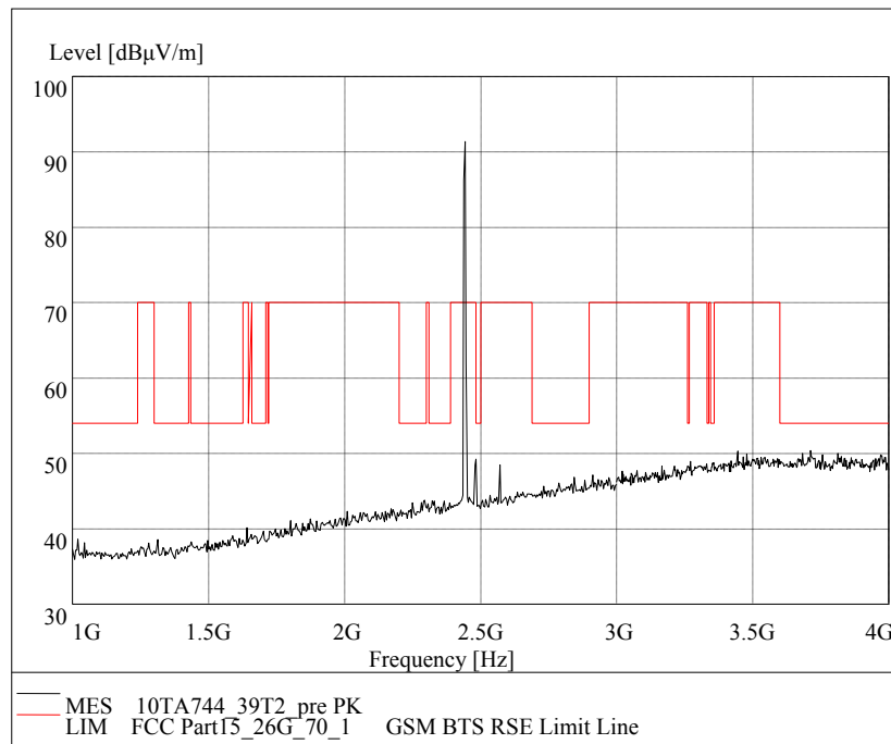
Fig.18 Radiated emission: GFSK, Channel 39, 1 GHz - 4 GHz
