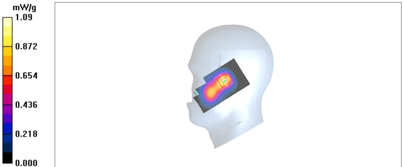
Fig. 25 1900 MHz CH512
