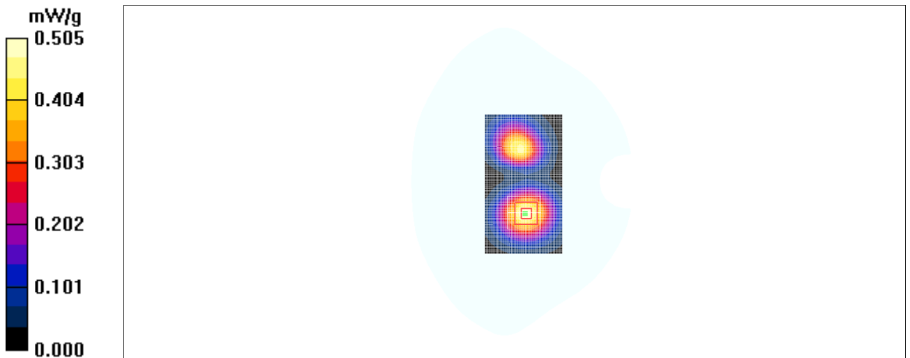
Fig. 39 1900 MHz CH512
