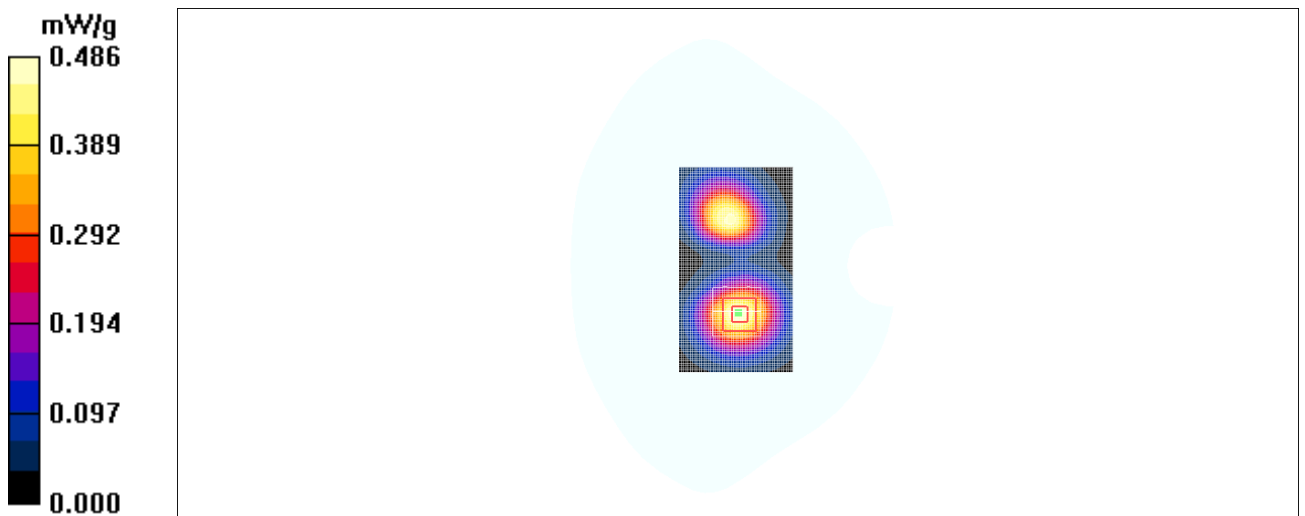
Fig. 38 1900 MHz CH661
