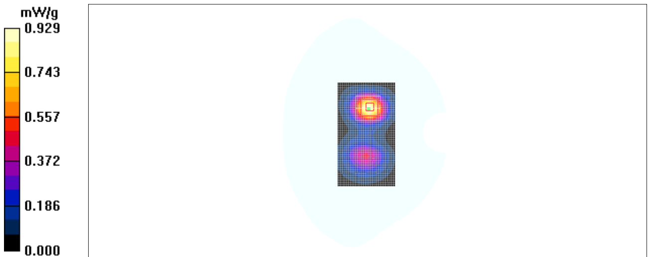
Fig. 35 1900 MHz CH661
