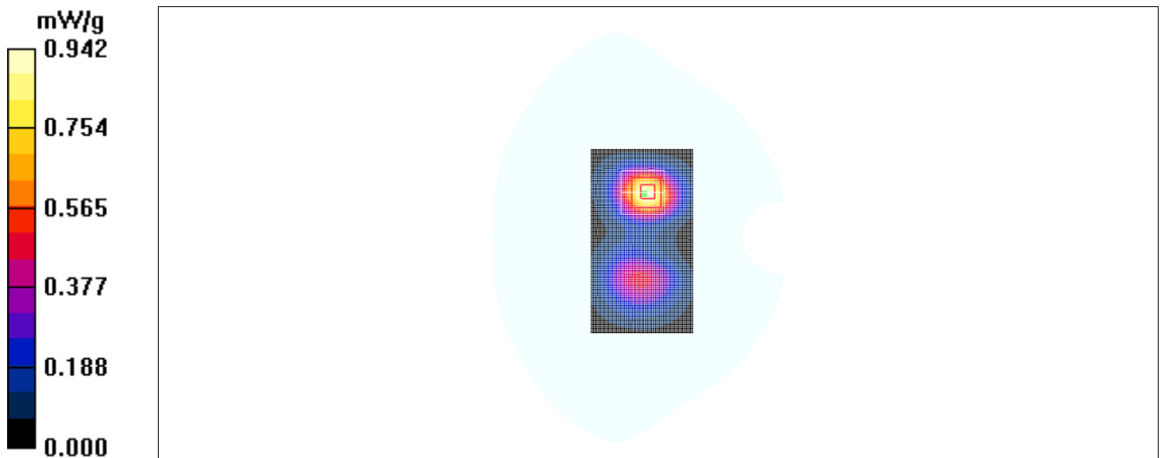
Fig. 36 1900 MHz CH512
