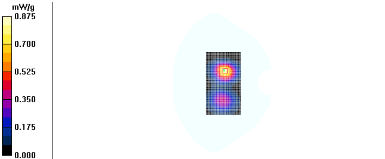
Fig. 41 1900 MHz CH512
