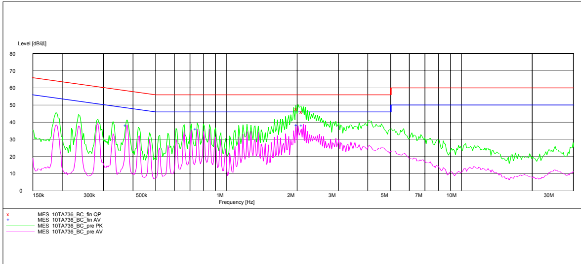
Fig.37 AC Powerline Conducted Emission with charger
