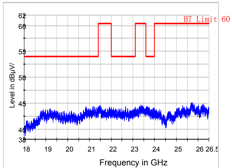
Fig.24 Radiated emission: GFSK, 18 GHz - 26 GHz
