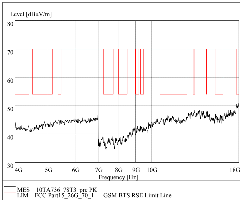
Fig.22 Radiated emission: GFSK, Channel 78, 4 GHz - 18 GHz
