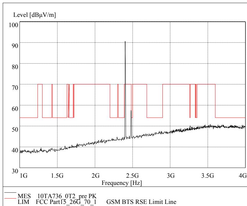
Fig.15 Radiated emission: GFSK, Channel 0, 1 GHz - 4 GHz
