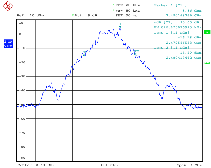
Fig.32 20dB Bandwidth: GFSK, Channel 39
