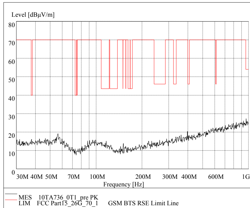
Fig.14 Radiated emission: GFSK, Channel 0, 30 MHz - 1 GHz
