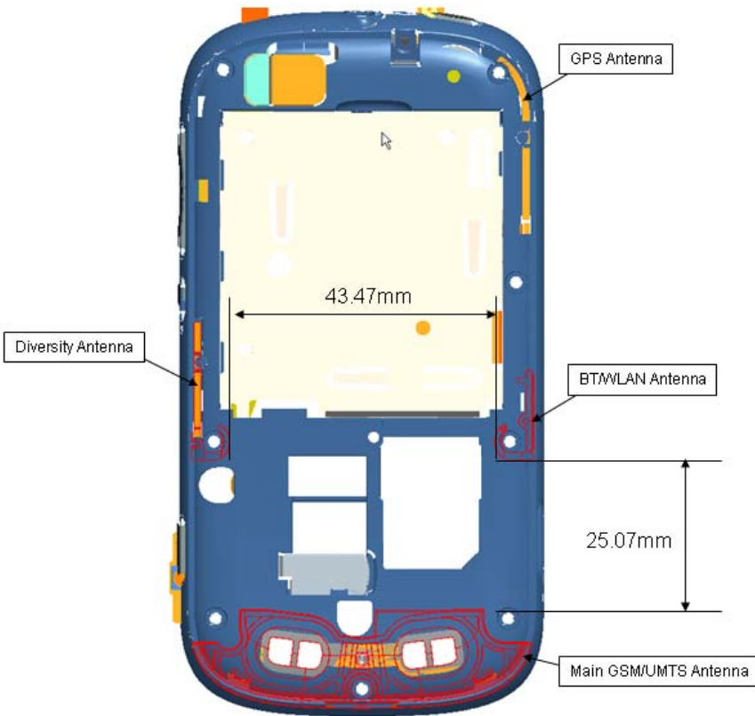
Figure 7: Antenna Separation Distance
