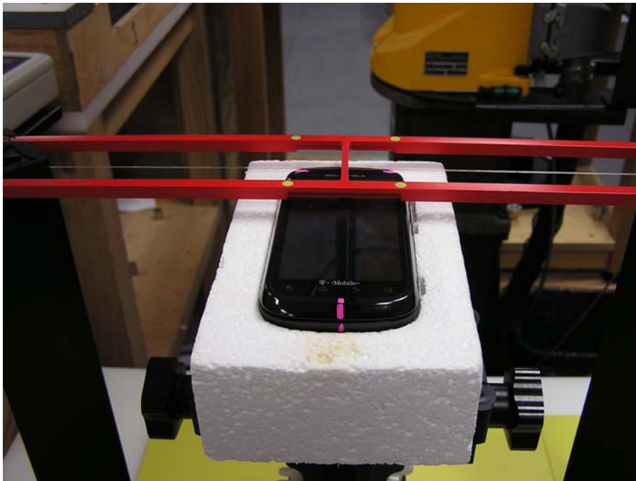
Figure 5. Positioning and Measurement for RF Emissions
