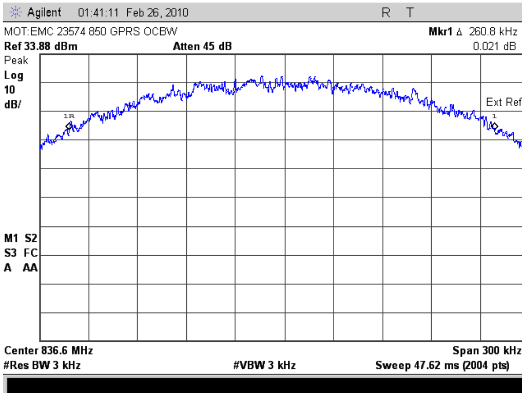
GSM 850 – Channel 190 (836.60 MHz) – Occupied Bandwidth
