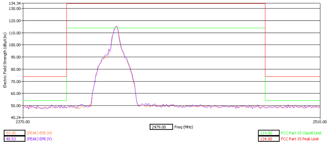
Low Band Edge Z Orientation
