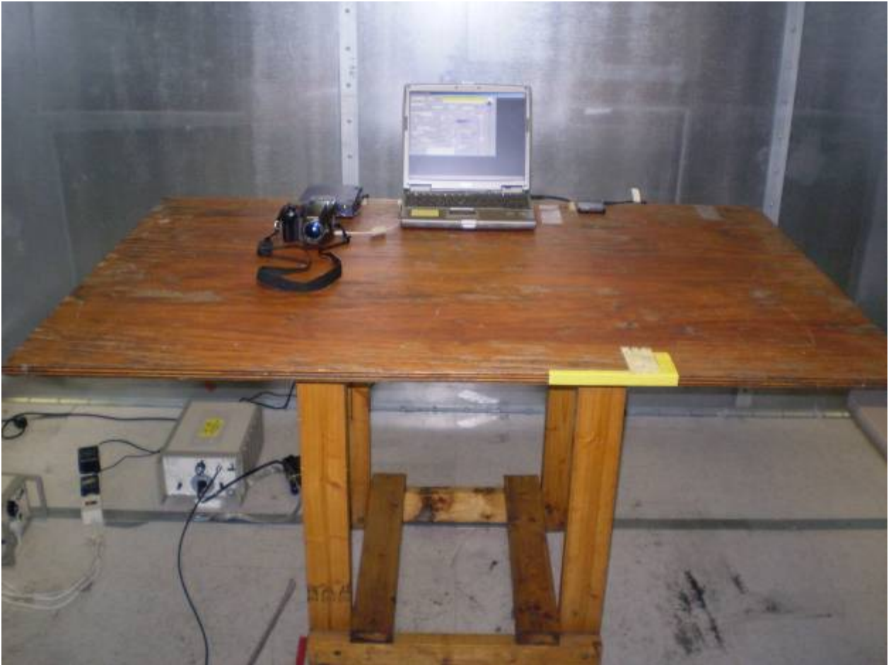
AC Line Conducted Emissions - Part 15 PC Peripheral
