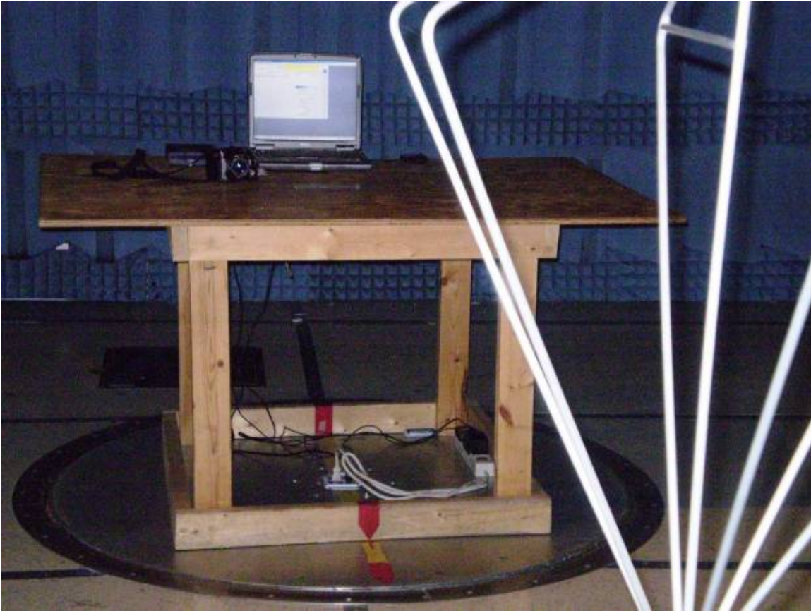
Radiated Emissions - Part 15 PC Peripheral
