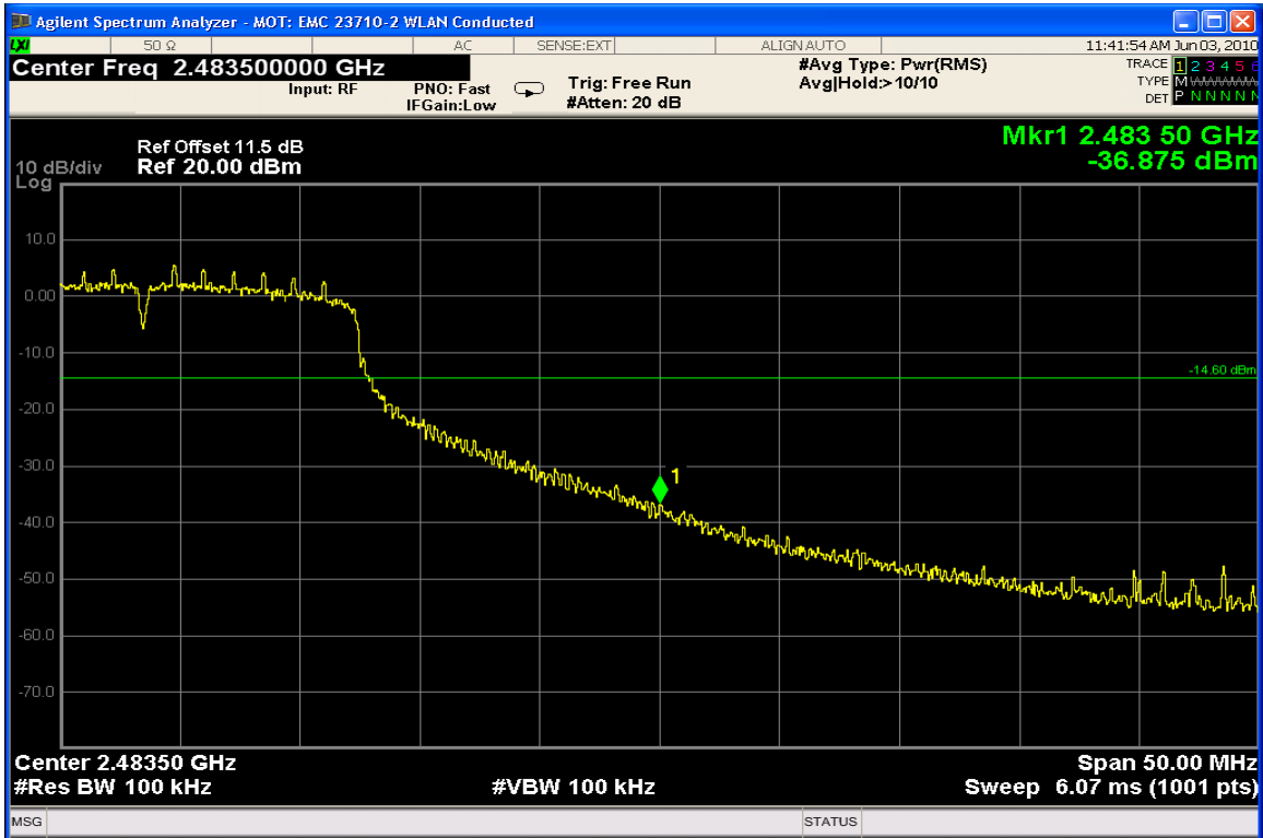
Channel 11 @ 7.2 Mbps – Upper Band Edge
