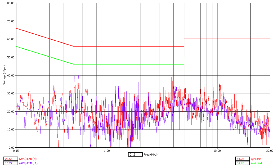
Bluetooth – Hopping - Tx Mode – AVG Detector
