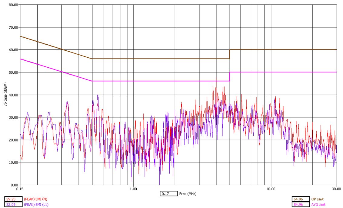
Bluetooth – Hopping - Tx Mode – Peak Detector
