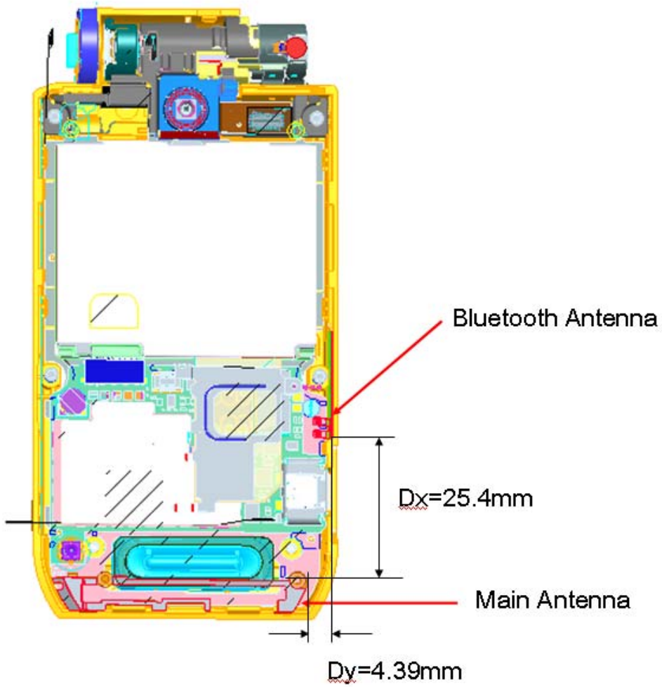
Figure 7: Antenna Separation Distances
