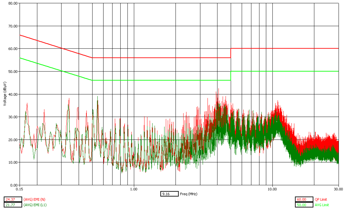
Bluetooth – Hopping - Tx Mode – AVG Detector
