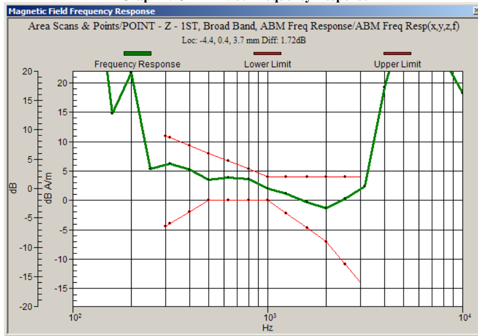
Graph 2: CDMA 1900 Frequency Response
