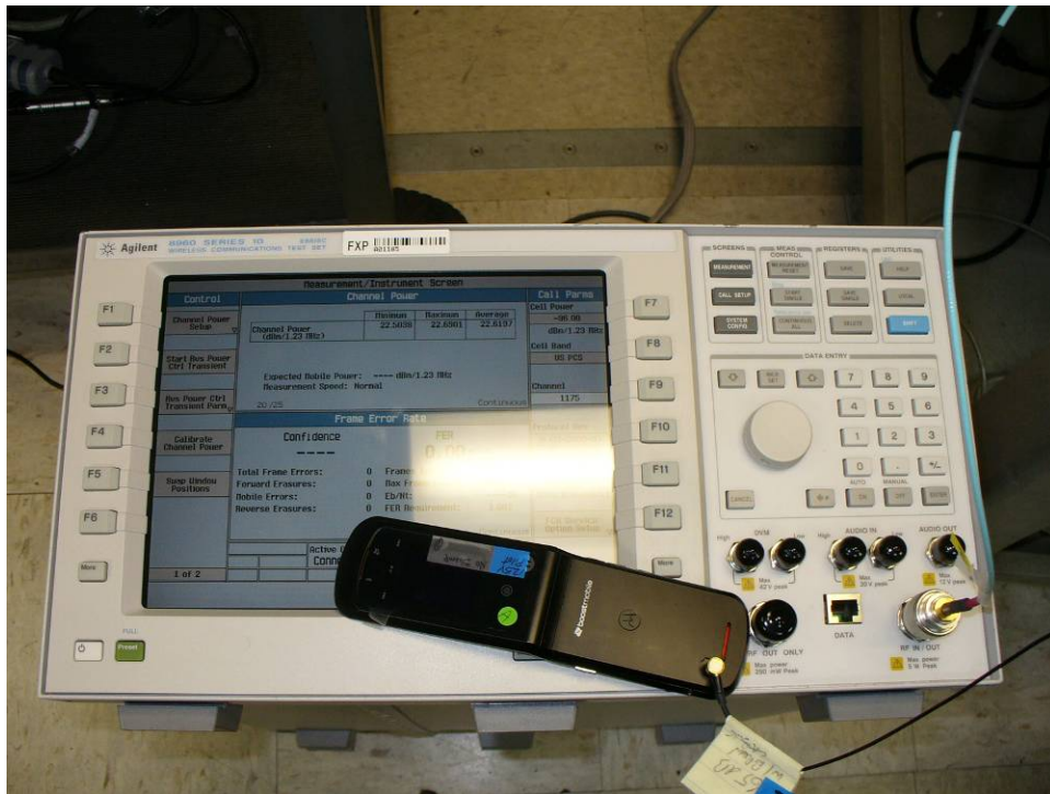
Photograph 10: Spurious Emissions at Antenna Terminals Setup (Close-up on EUT)
