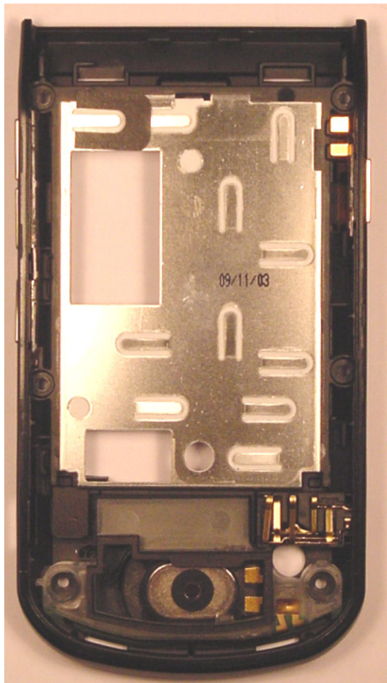
Base Outer Housing
