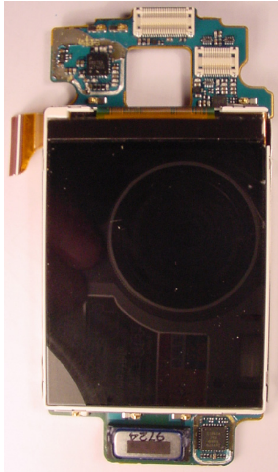
Flip Board without Shields
