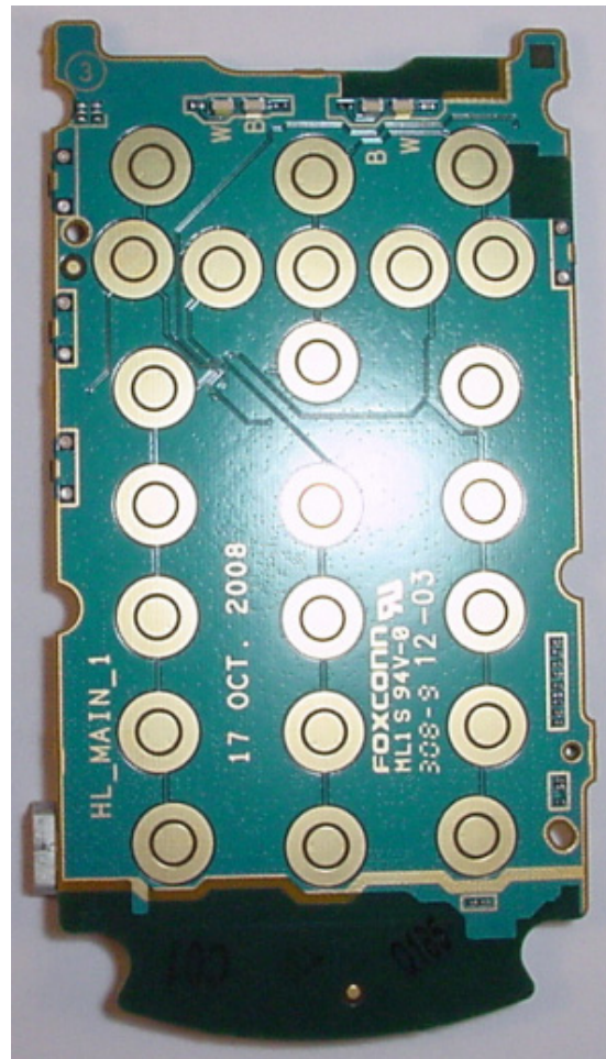
Main Board Top Without Popples
