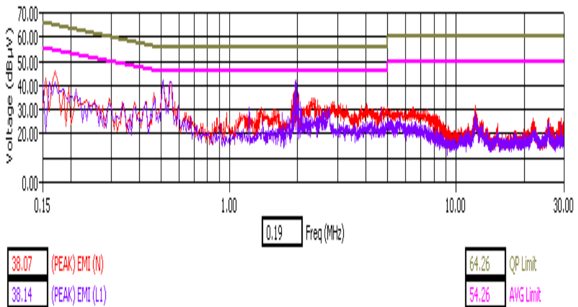
Bluetooth – Hopping - Tx Mode – Peak Detector
