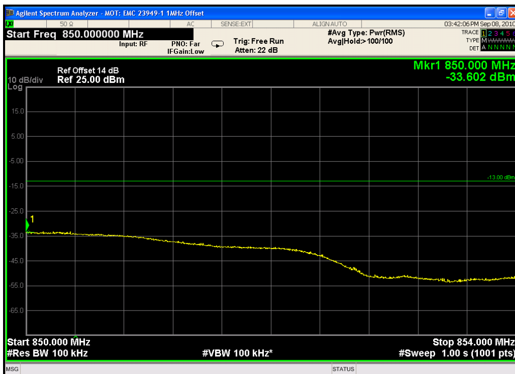
BandV WCDMA Conducted Spurious Emissions (Upper adjacent 100 kHz band)
