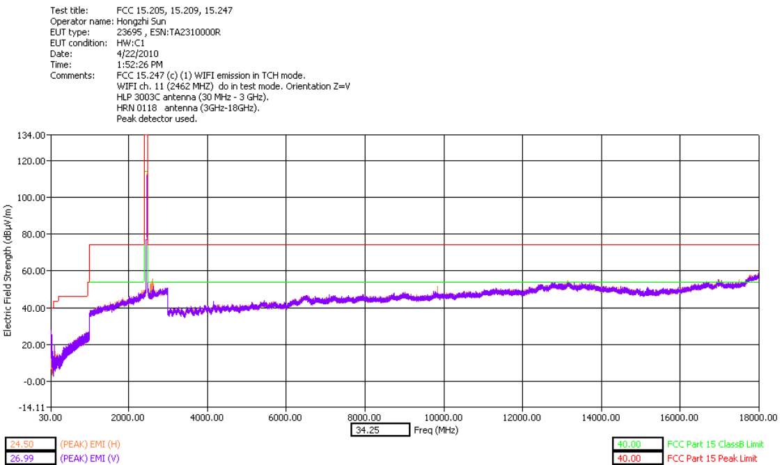
30 - 18000MHz High Channel Dual Polarization Z
