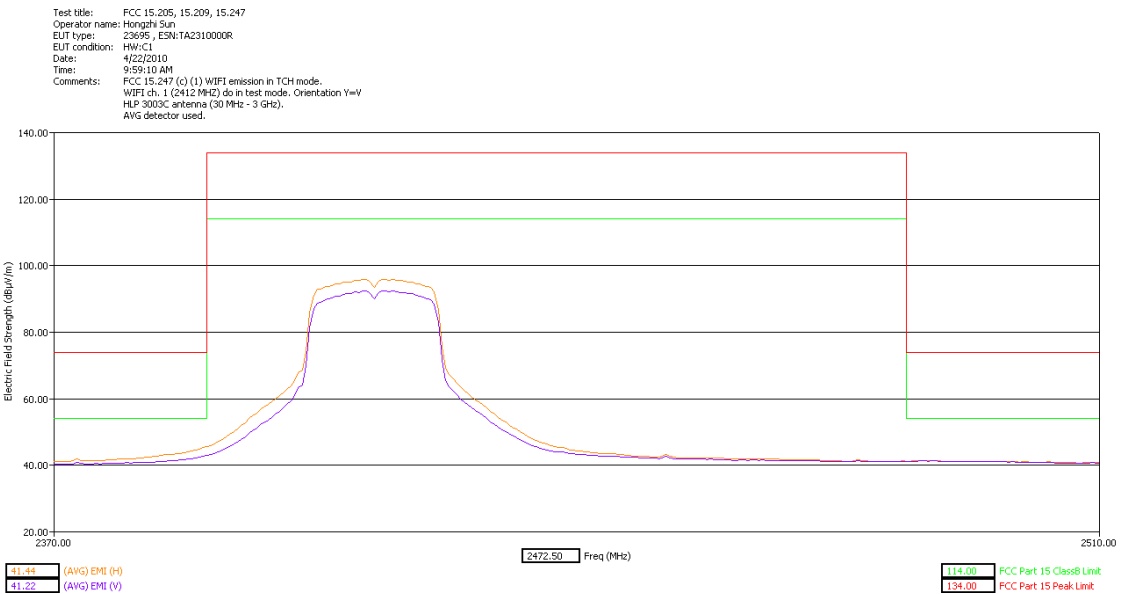
Low Band Edge Y Orientation
