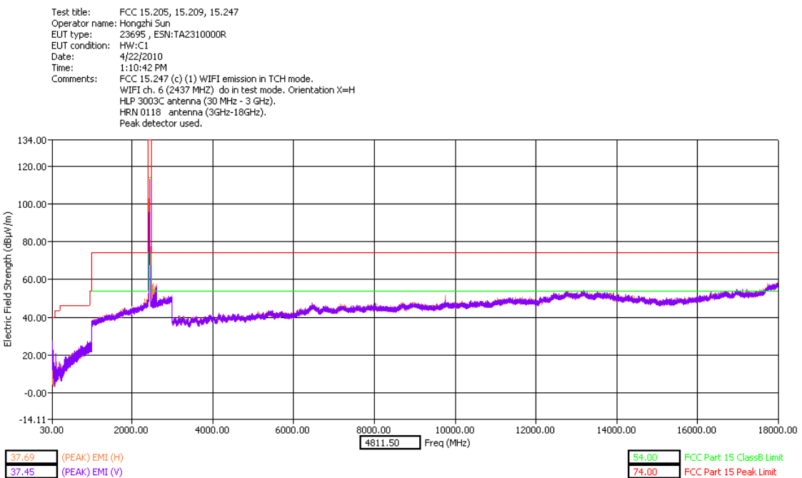
30 - 18000MHz Middle Channel Dual Polarization X
