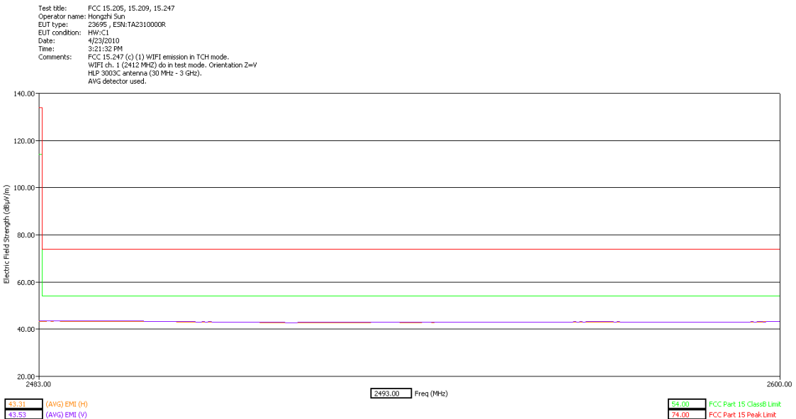
Emissions from 2483 MHz to 2600 MHz Low channel Polarization Z
