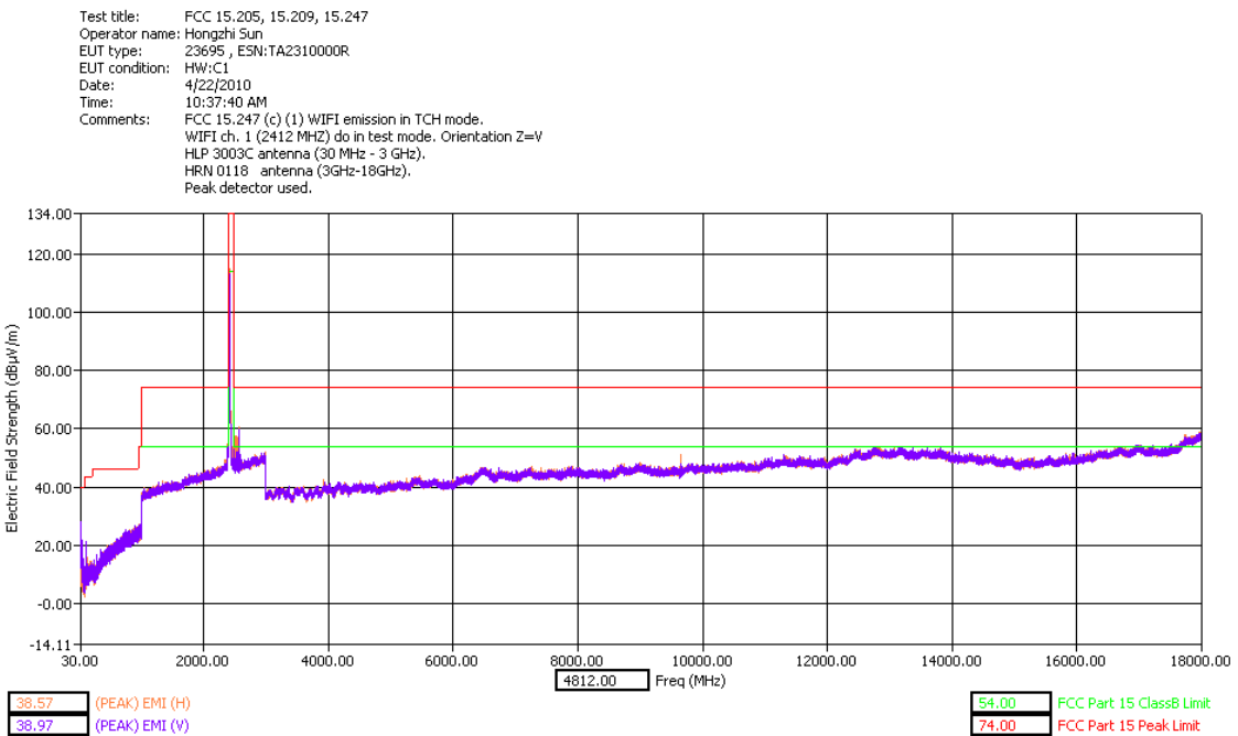
30 - 18000MHz Low Channel Dual Polarization Z
