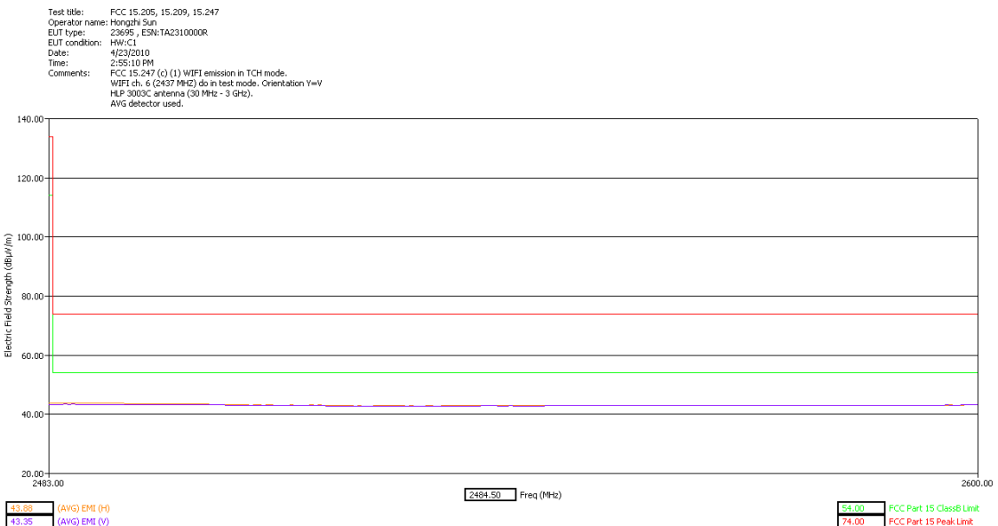
Emissions from 2483 MHz to 2600 MHz mid channel Polarization Y
