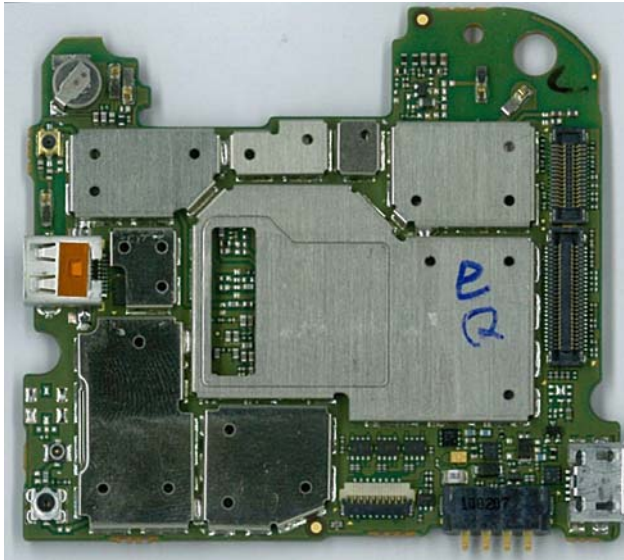
Main Board Bottom W/ Shields
