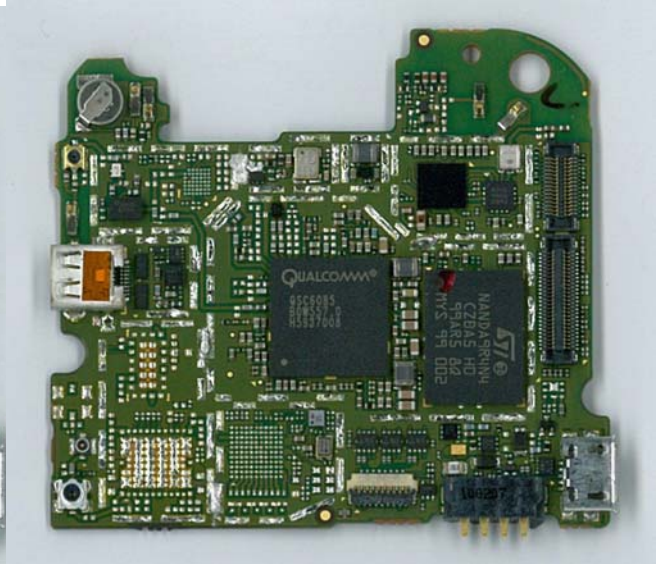
Main Board Bottom W/O Shields
