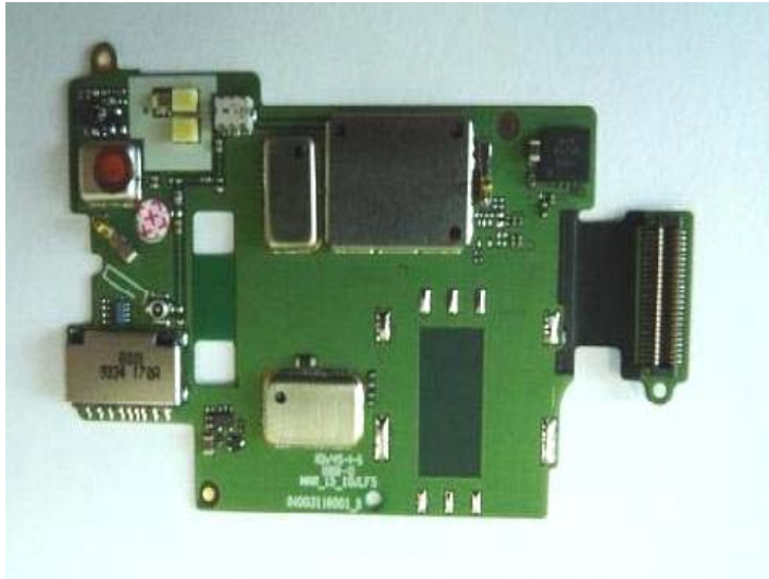
Daughter Board Top W/ shields
