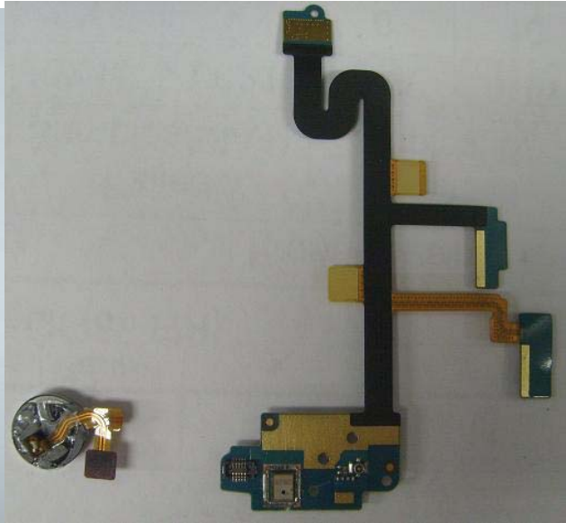
Vibrator Acoustic PCB Bottom W/O Shield
