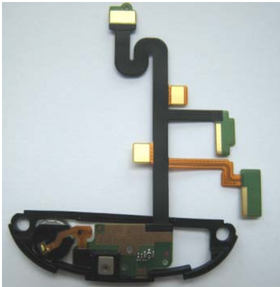
Linear Acoustic PCB Bottom W/ Shield
