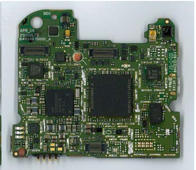
Main Board Top W/O shields
