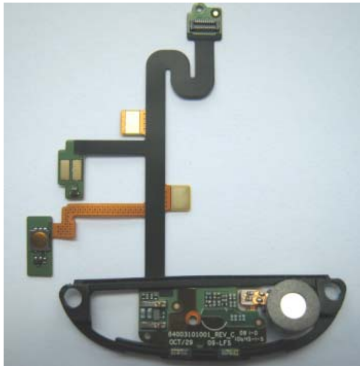
Acoustic PCB Top
